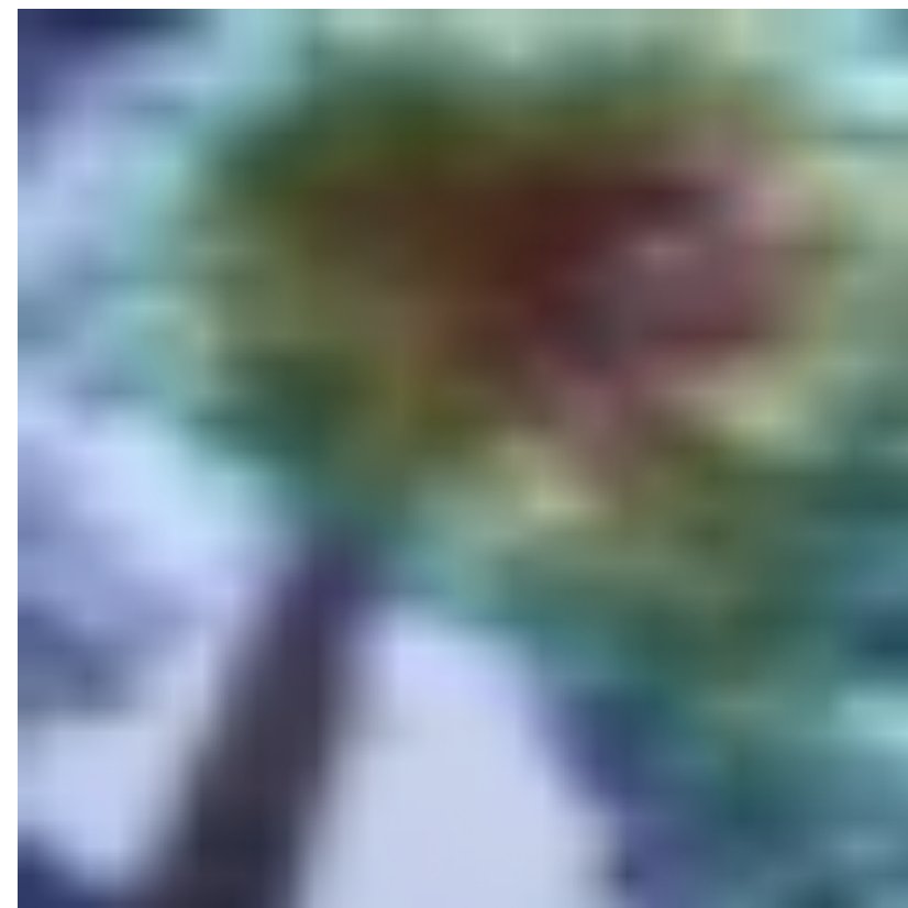
ResNet18
