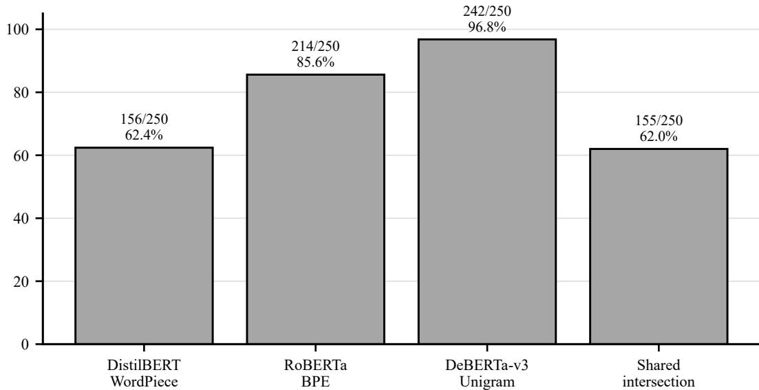
Clean toxic examples eligible (%)
