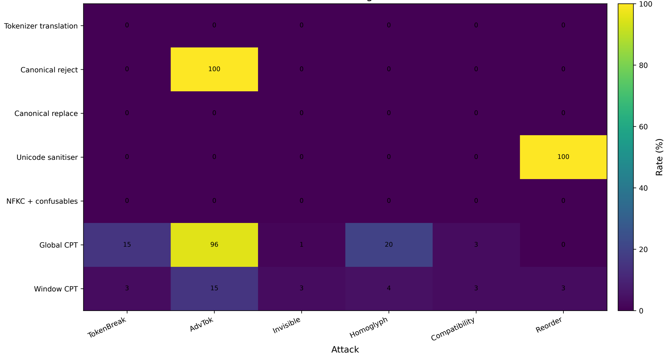
Attack blocking rate
