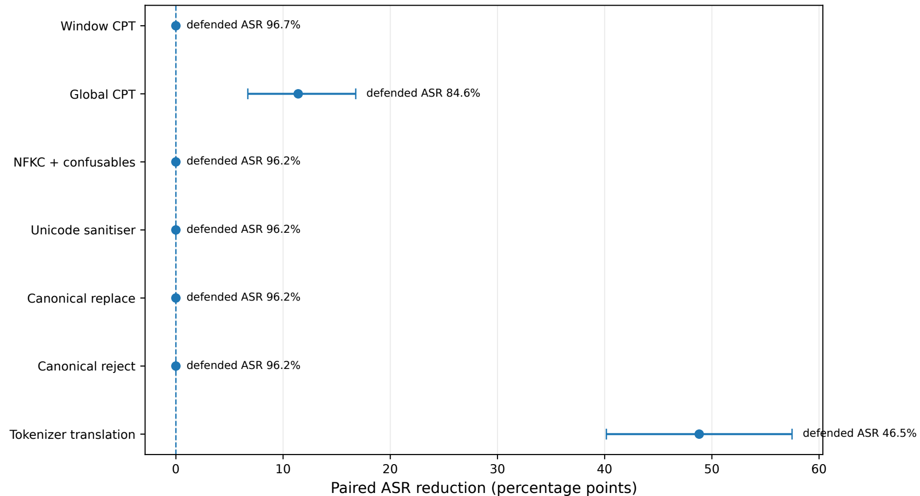
TokenBreak defence effectiveness with 95% confidence intervals
