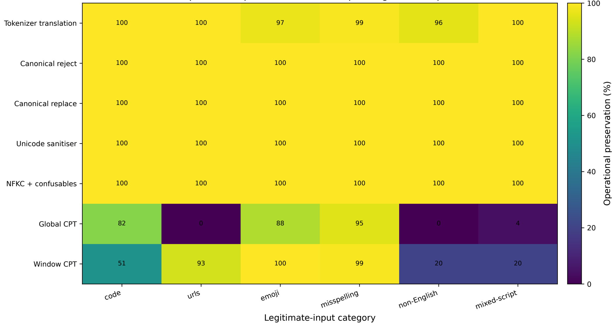
Operational preservation on complex legitimate inputs
