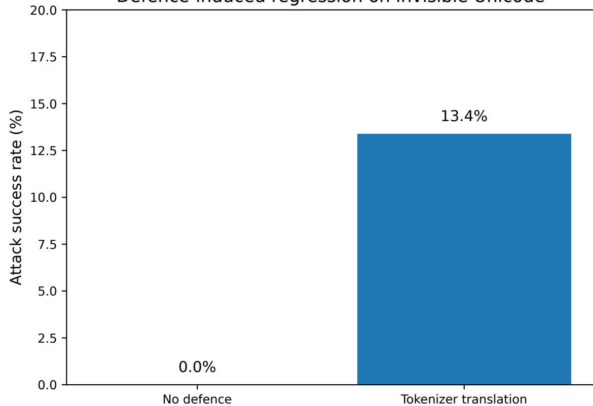
Defence-induced regression on invisible Unicode
