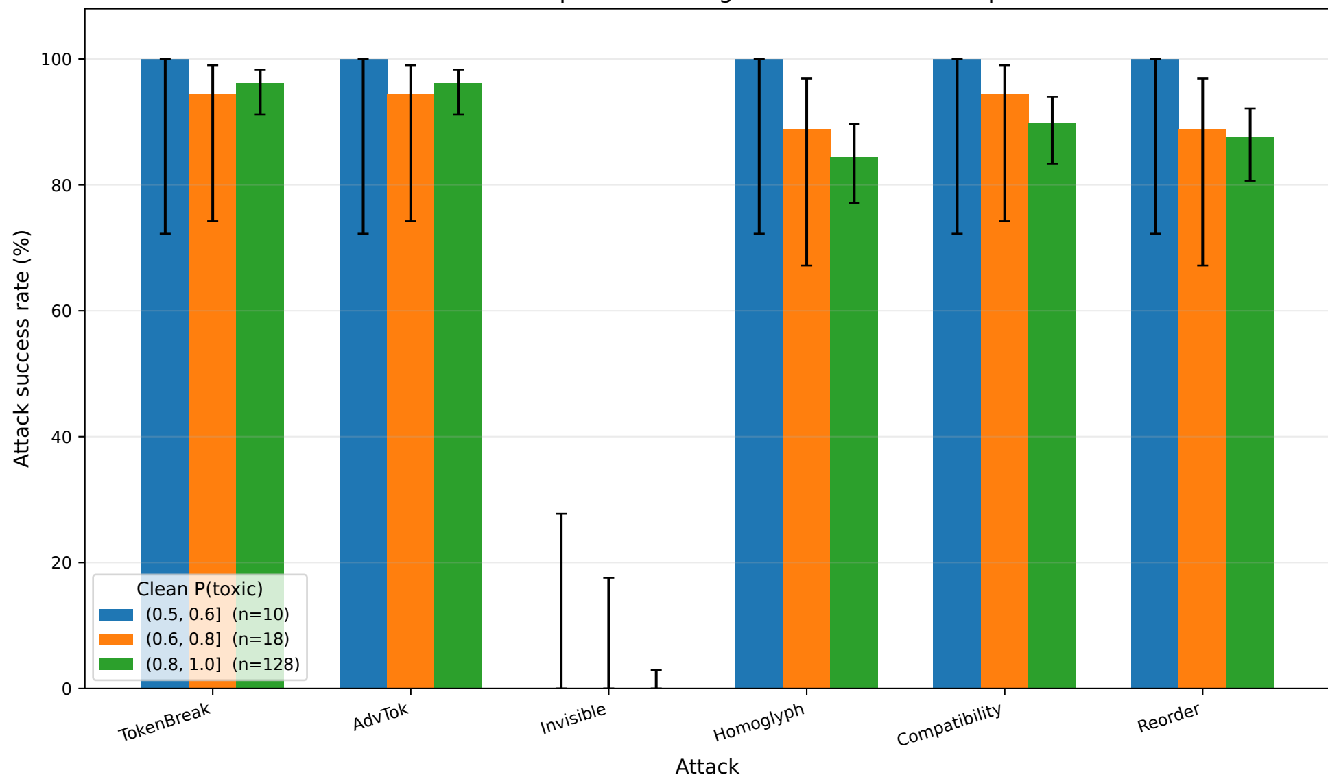
Attack success persists on high-confidence clean inputs
