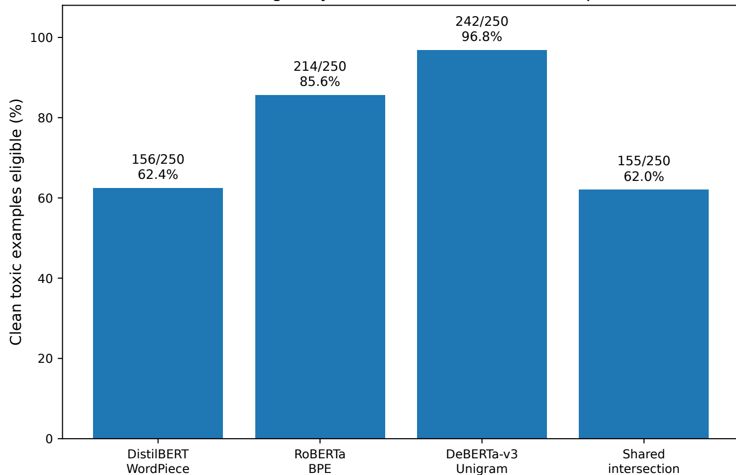
Clean eligibility across model-tokenizer setups
