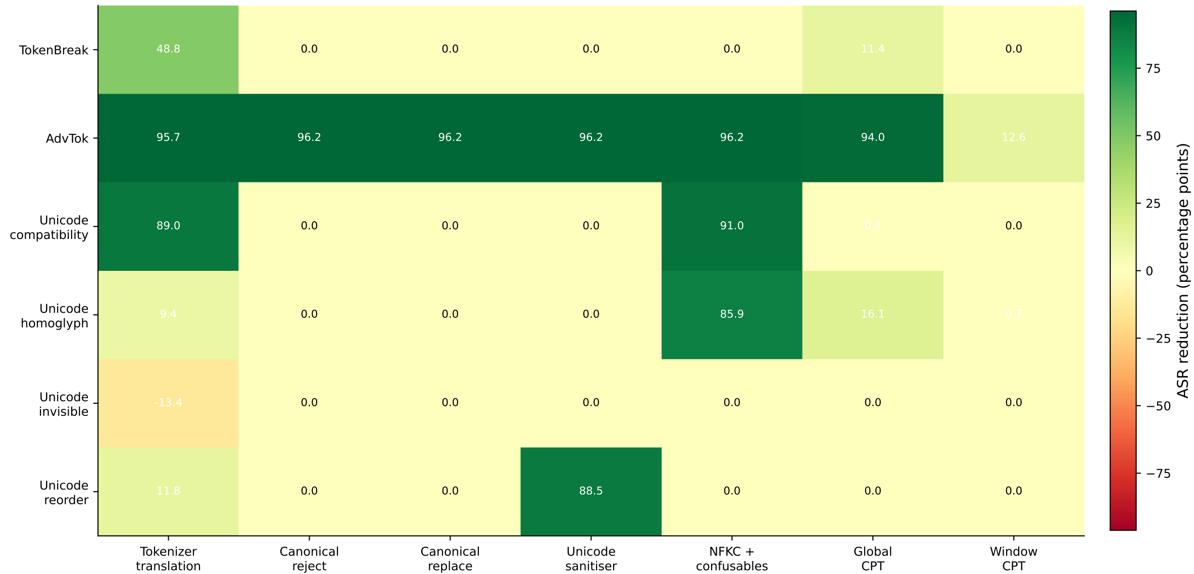
Change in attack success after defence
