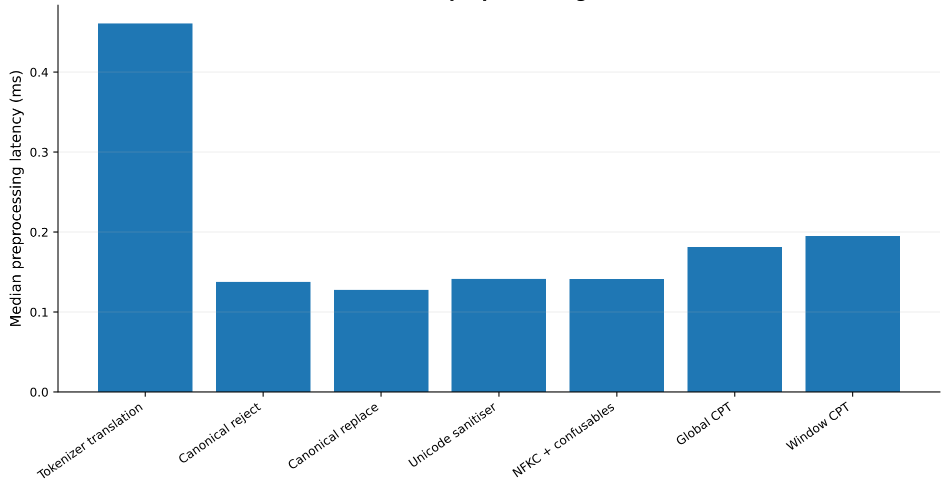
Defence preprocessing cost
