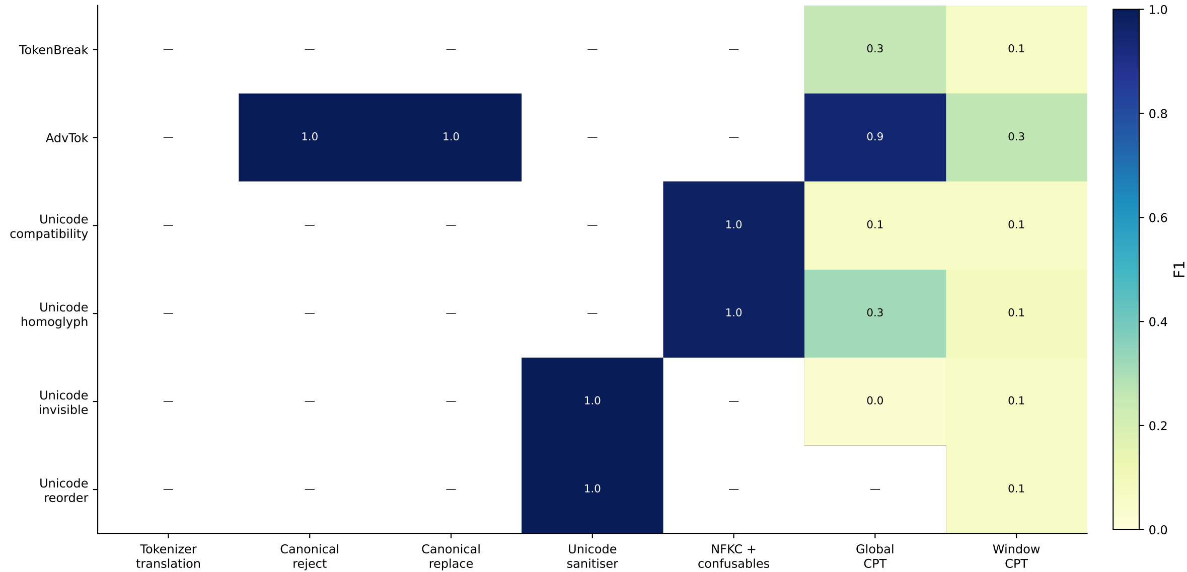
Flag-based attack-detection F1 against jigsaw benign controls
