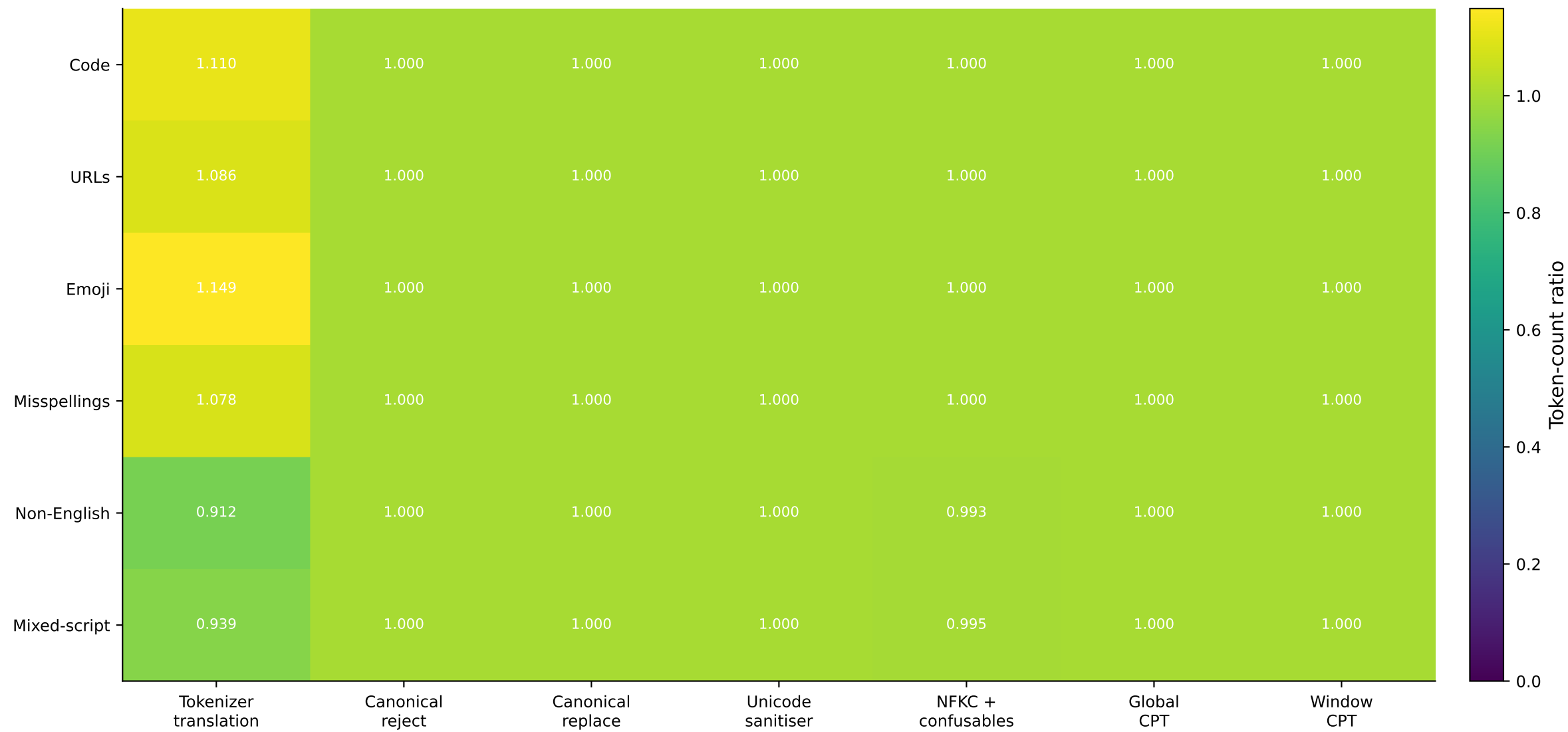
Mean defended / canonical token-count ratio
