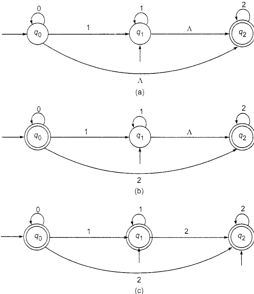
Fig. 5.2 Transition system for Example 5.5, without \Lambda -moves.
