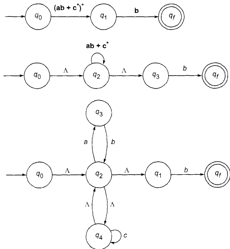
Fig. A5.3 Transition system for Exercise 5.9.
