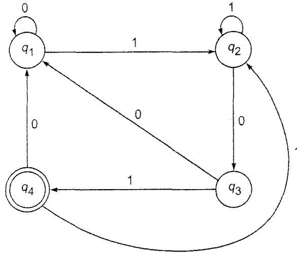
Fig. 5.17 Finite automaton of Example 5.12.
