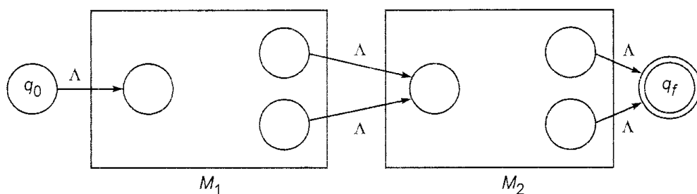
Fig. 5.8 NFA accepting L(PQ) .
