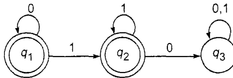
Fig. 5.15 Finite automaton of Example 5.10.
