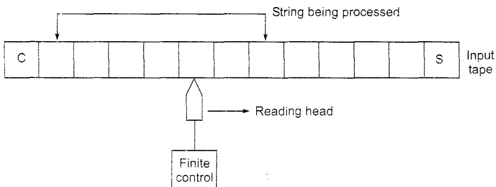
Fig. 3.4 Block diagram of a finite automaton.
