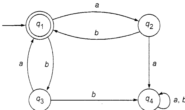
Fig. 5.14 Finite automaton of Example 5.9.
