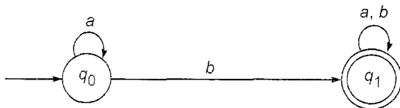
Fig. 5.32 DFA of Example 5.24, without \Lambda -moves.
