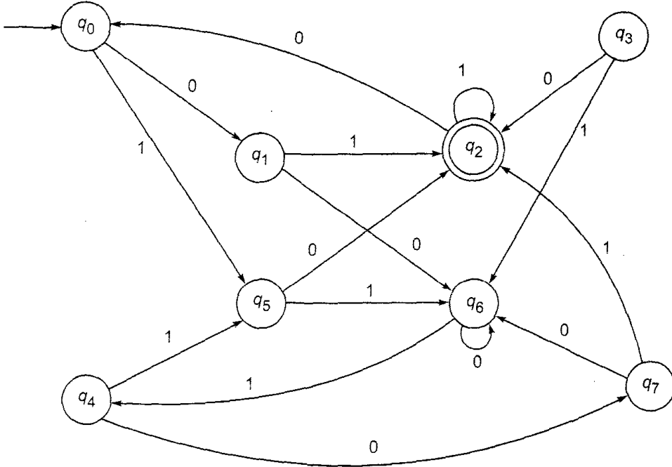
Fig. 3.12 Finite automaton of Example 3.13.
