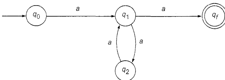
Fig. 5.28 Finite automaton of Example 5.22.
