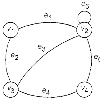
Fig. 2.3 An undirected graph.
