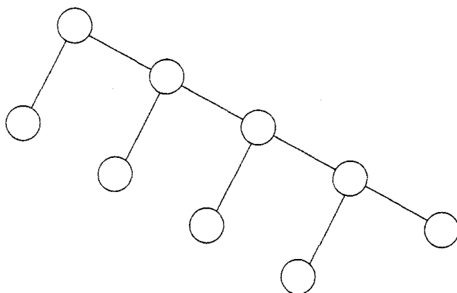
Fig. 2.12 Binary tree of maximum height with 9 vertices.
