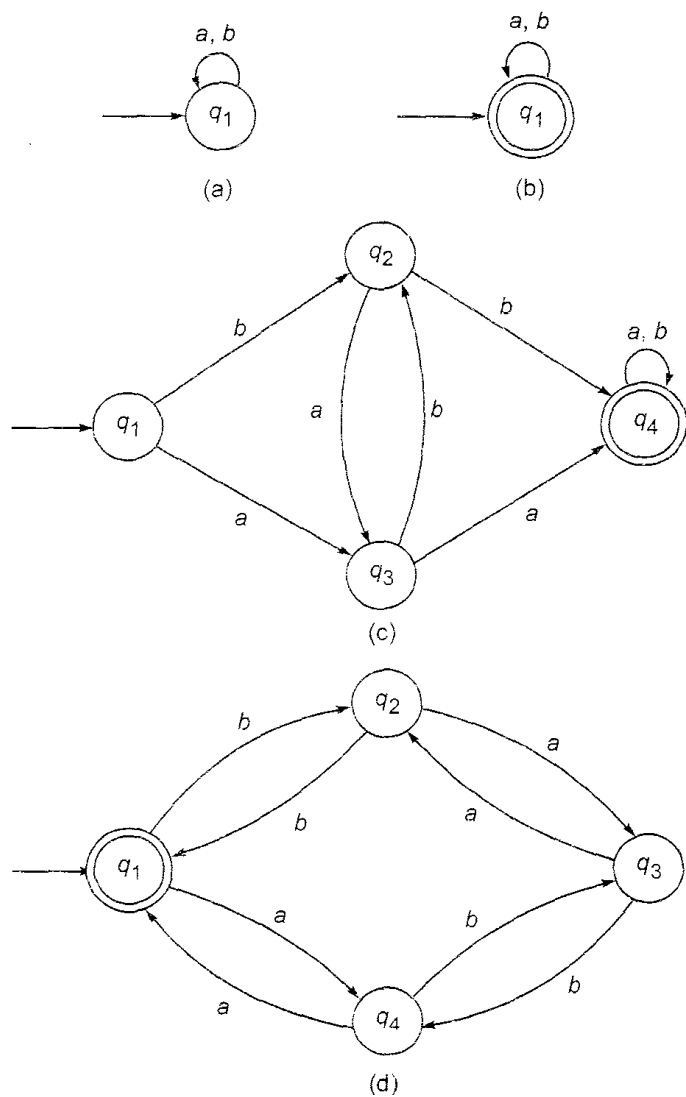
Fig. 5.37 Transition systems of Exercise 5.7.
