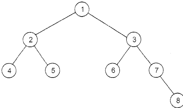
Fig. 2.18 The tree for Exercise 2.15.
