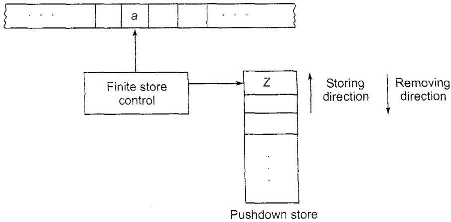
Fig. 7.1 Model of a pushdown automaton.
