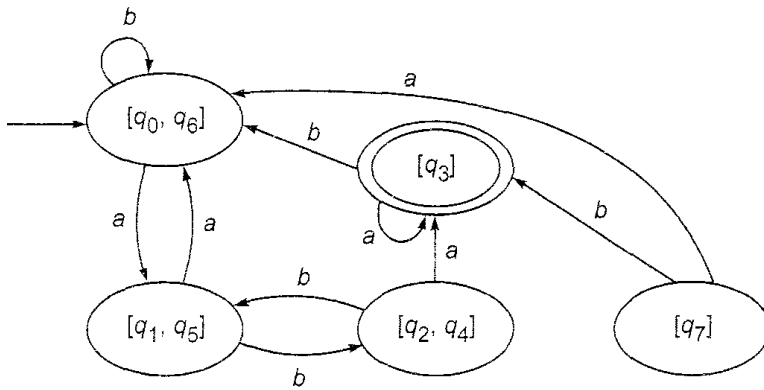
Fig. 3.15 Minimum state automaton of Example 3.14.
