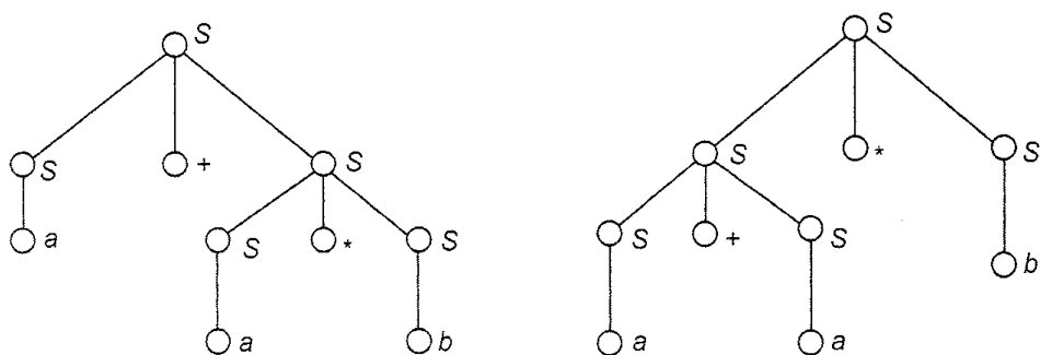
Fig. 6.10 Two derivation trees for a + a * b .
