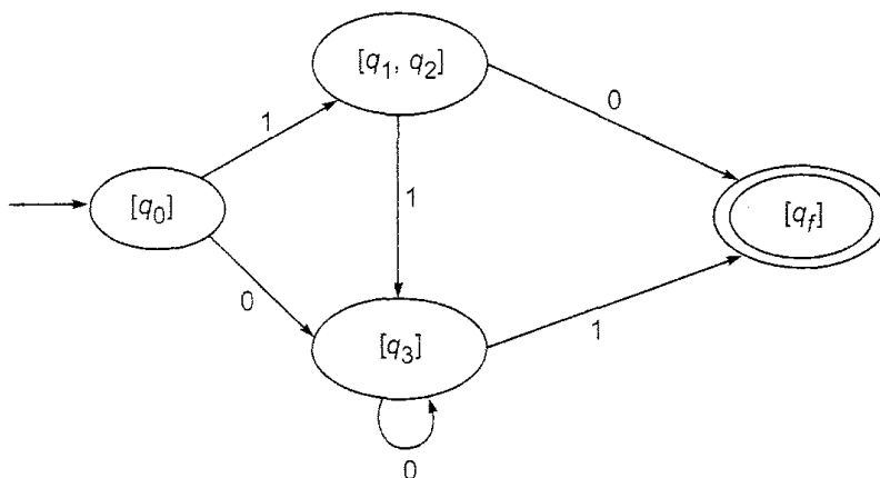
Fig. 5.22 Reduced DFA of Example 5.14.
