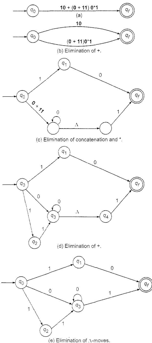
Fig. 5.21 Construction of finite automaton for Example 5.14.
