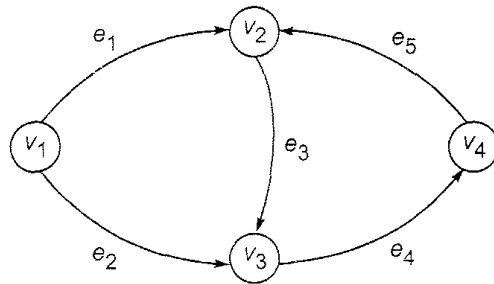
Fig. 2.4 A directed graph.
