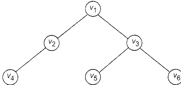
Fig. 2.9 Representation of an ordered directed tree.
