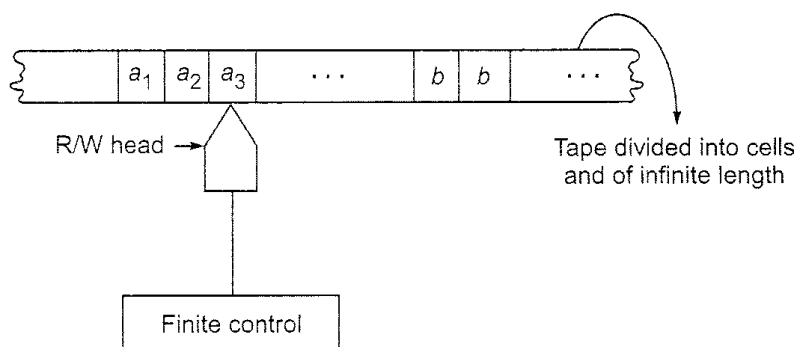
Fig. 9.1 Turing machine model.
