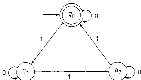
Fig. 3.20 Automaton for Questions 1–5.
