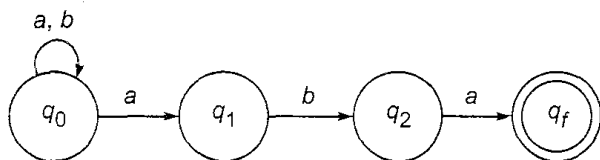
Fig A5.5 Transition system for Exercise 5.24.
