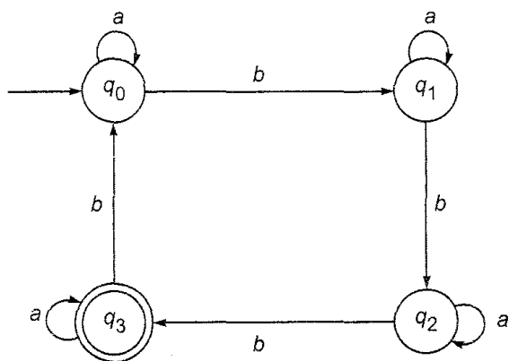
Fig. 5.35 DFA for Example 5.35.
