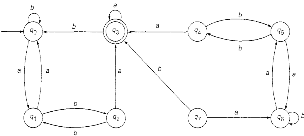
Fig. 3.14 Finite automaton of Example 3.14.
