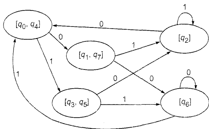
Fig. 3.13 Minimum state automaton of Example 3.13.
