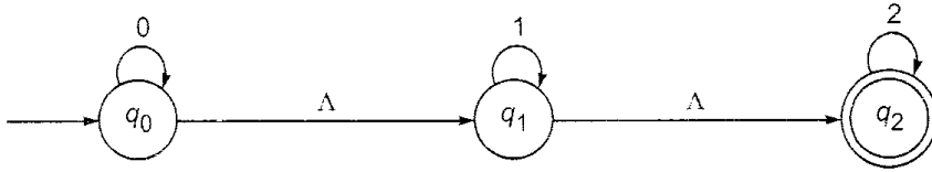
Fig. 5.1 Finite automaton of Example 5.5.
