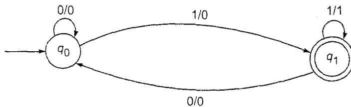
Fig. 3.5 A transition system.
