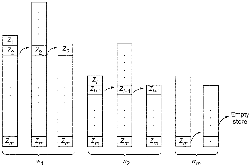
Fig. 7.3 Illustration of changes in pushdown store.
