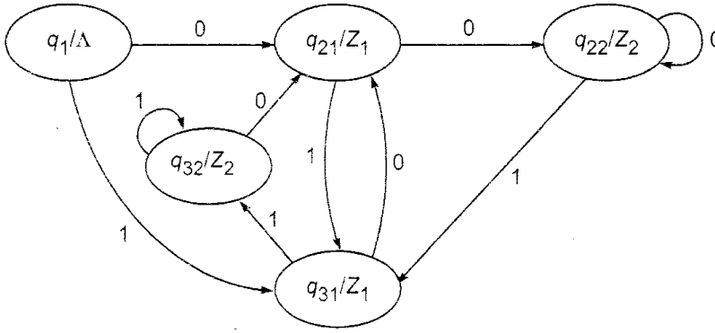
Fig. 3.11 Moore machine of Example 3.12.
