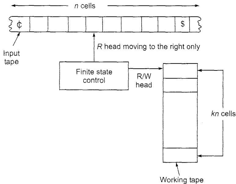
Fig. 9.11 Model of linear bounded automaton.
