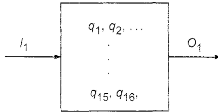
Fig. 3.3 A shift register as a finite-state machine.
