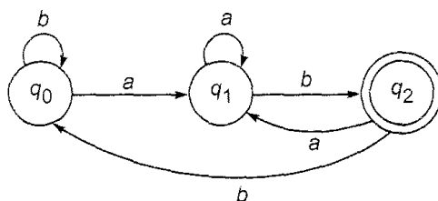
Fig. 3.19 DFA of Example 3.19.
