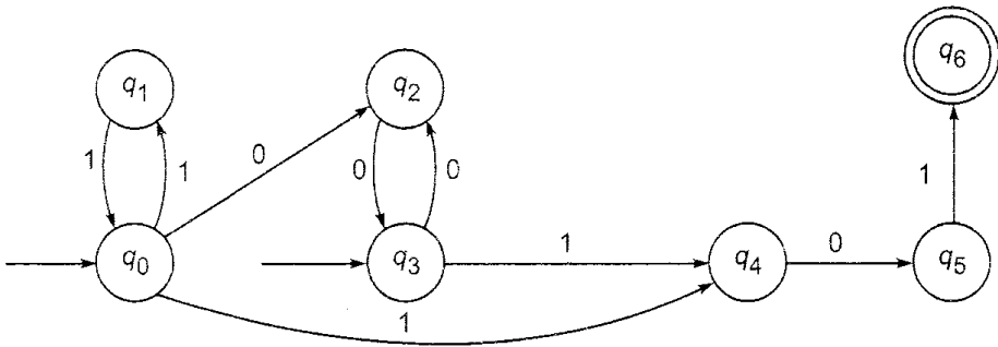
Fig. 5.4 Transition system for Example 5.6, without \Lambda -moves.
