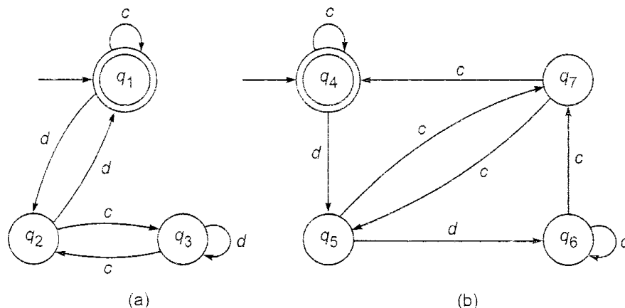
Fig. 5.24 (a) Automaton M_1 and (b) automaton M_2 .
