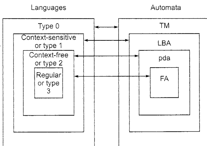
Fig. 4.1 Languages and the corresponding automata.
