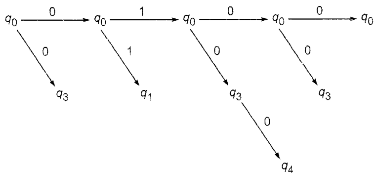
Fig. 3.9 States reached while processing 0100.
