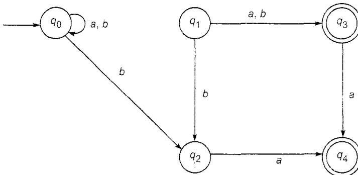
Fig. 3.16 NFA of Example 3.15.
