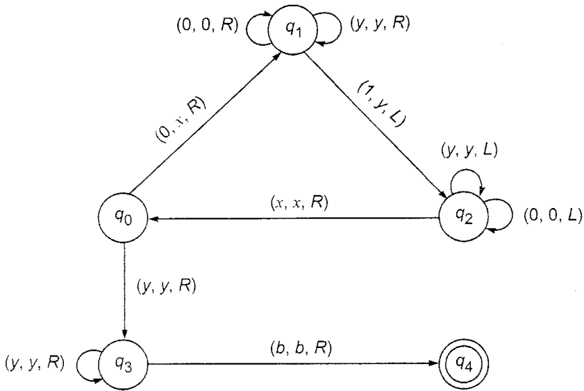
Fig. 9.7 Transition diagram for Example 9.7.
