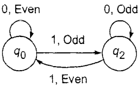
Fig. A3.3 Mealy machine of Exercise 3.13.
