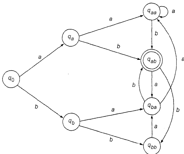
Fig. 3.18 DFA of Example 3.18.
