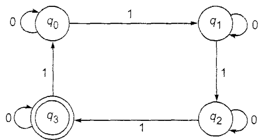
Fig. 3.17 DFA of Example 3.17.
