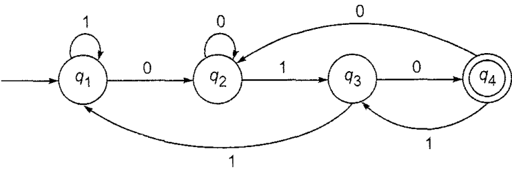
Fig. 9.12 DFA for Example 9.14.
