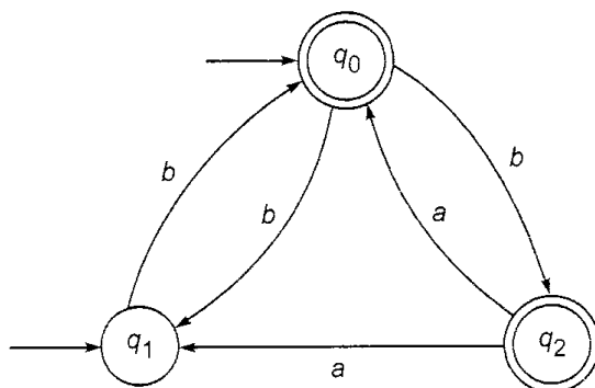
Fig. 5.11 Nondeterministic transition system of Example 5.7.
