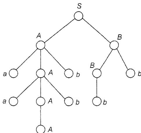
Fig. 8.1 Derivation tree for a^2b^4 .
