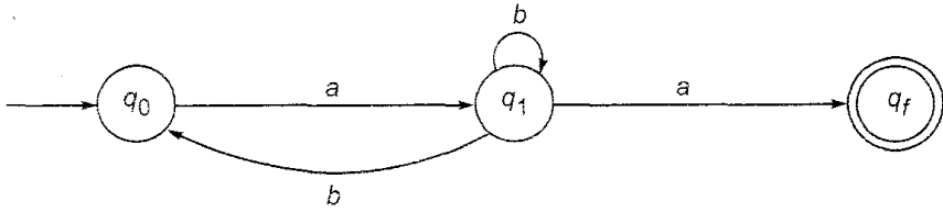
Fig. 5.33 Transition system for Example 5.25.
