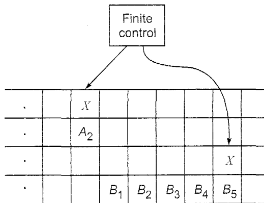
Fig. 9.9 Simulation of multitape TM.
