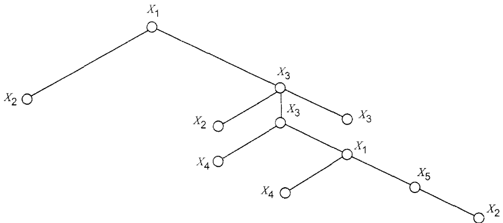
Fig. 6.15 Derivation tree for Exercise 6.3.
