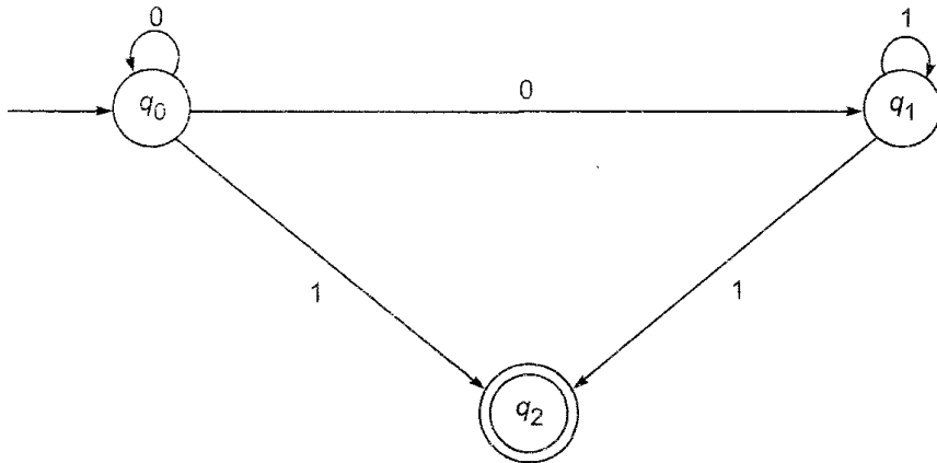
Fig. 3.7 Transition system representing nondeterministic automaton.
