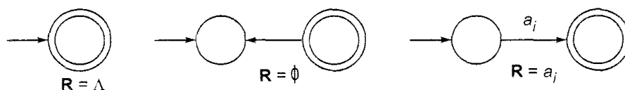
Fig. 5.5 Transition systems for recognizing elementary regular sets.
