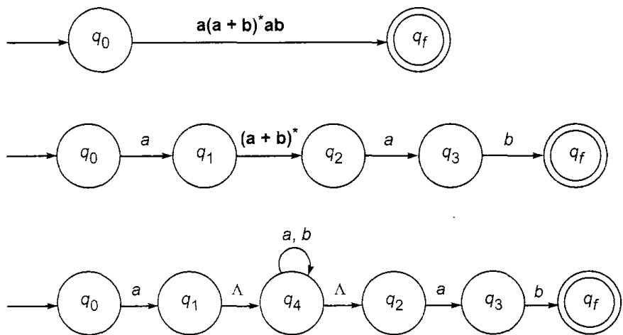
Fig. A5.2 Transition system for Exercise 5.6.
