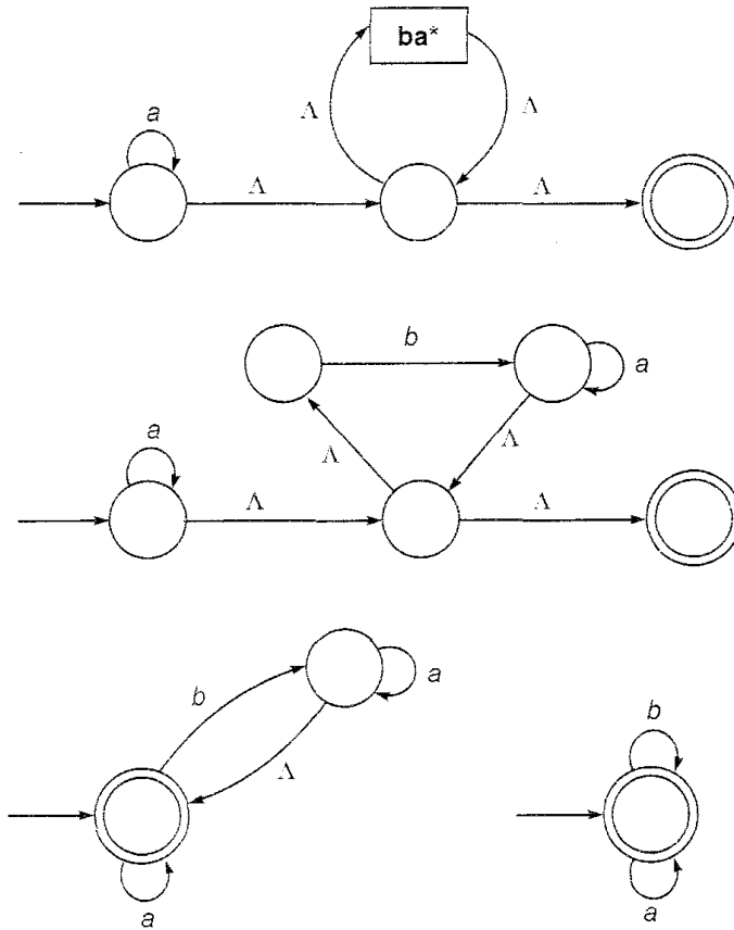
Fig. 5.26 Transition system for a^*(ba^*)^* .
