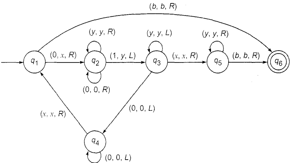
Fig. 9.4 Transition system for M .
