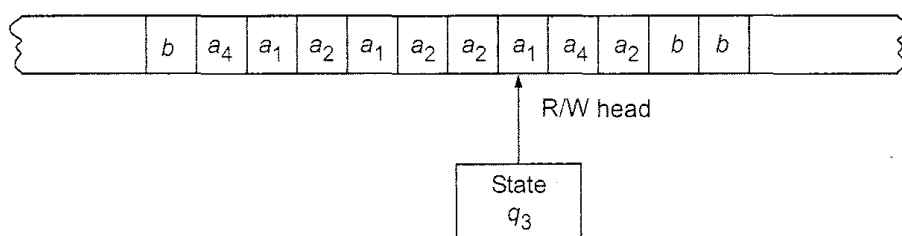
Fig. 9.2 A snapshot of Turing machine.
