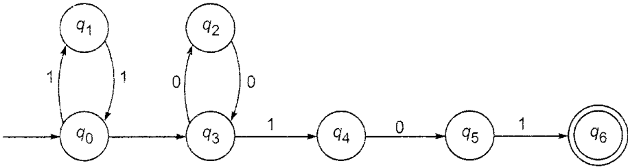
Fig. 5.3 Finite automaton of Example 5.6.
