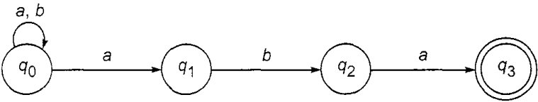
Fig. A3.1 NDFA for Exercise 3.6.
