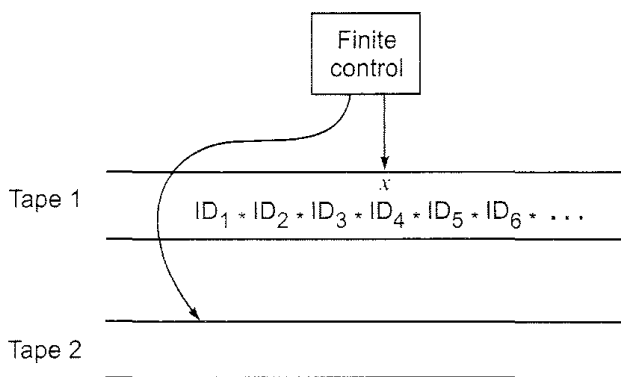
Fig. 9.10 The deterministic TM simulating M .
