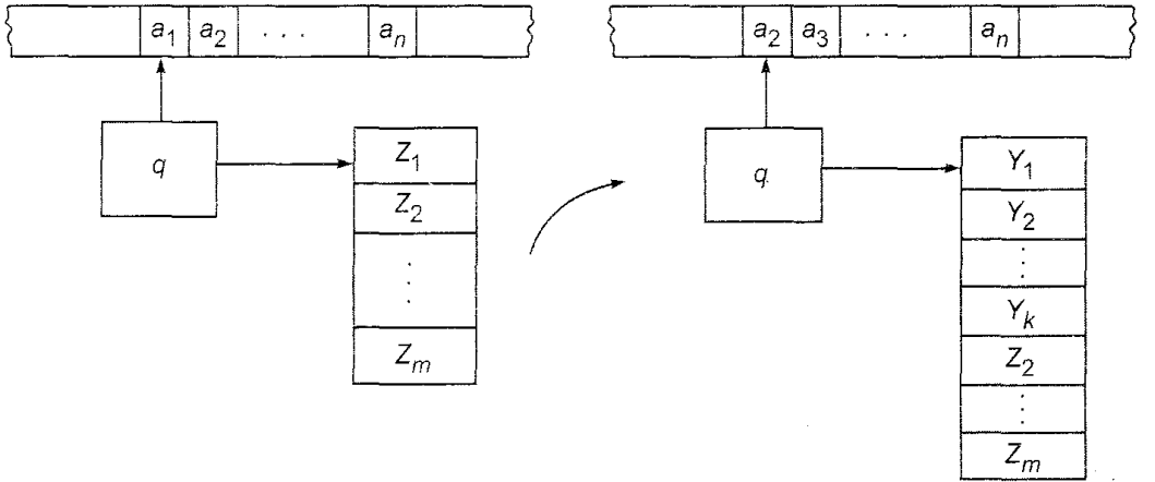
Fig. 7.2 An illustration of the move relation.
