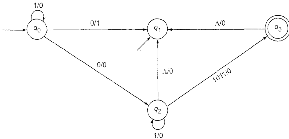
Fig. 3.6 Transition system for Example 3.2.
