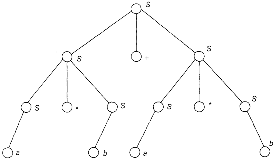
Fig. A6.1 Derivation tree for Exercise 6.1.
