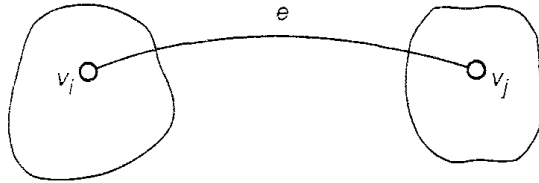
Fig. 2.16 Tree T with (n + 1) vertices.
