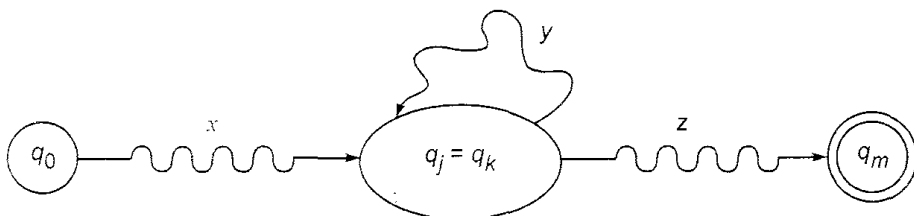
Fig. 5.27 String accepted by M .
