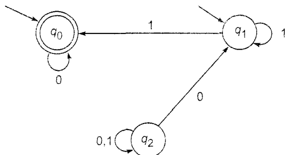
Fig. 5.30 Finite automaton of T(M)^T .
