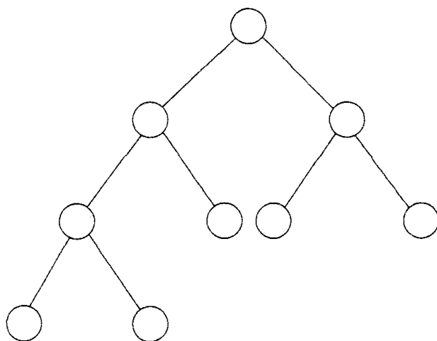
Fig. 2.11 Binary tree of minimum height with 9 vertices.
