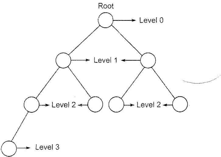
Fig. 2.10 Illustration of levels of vertices.
