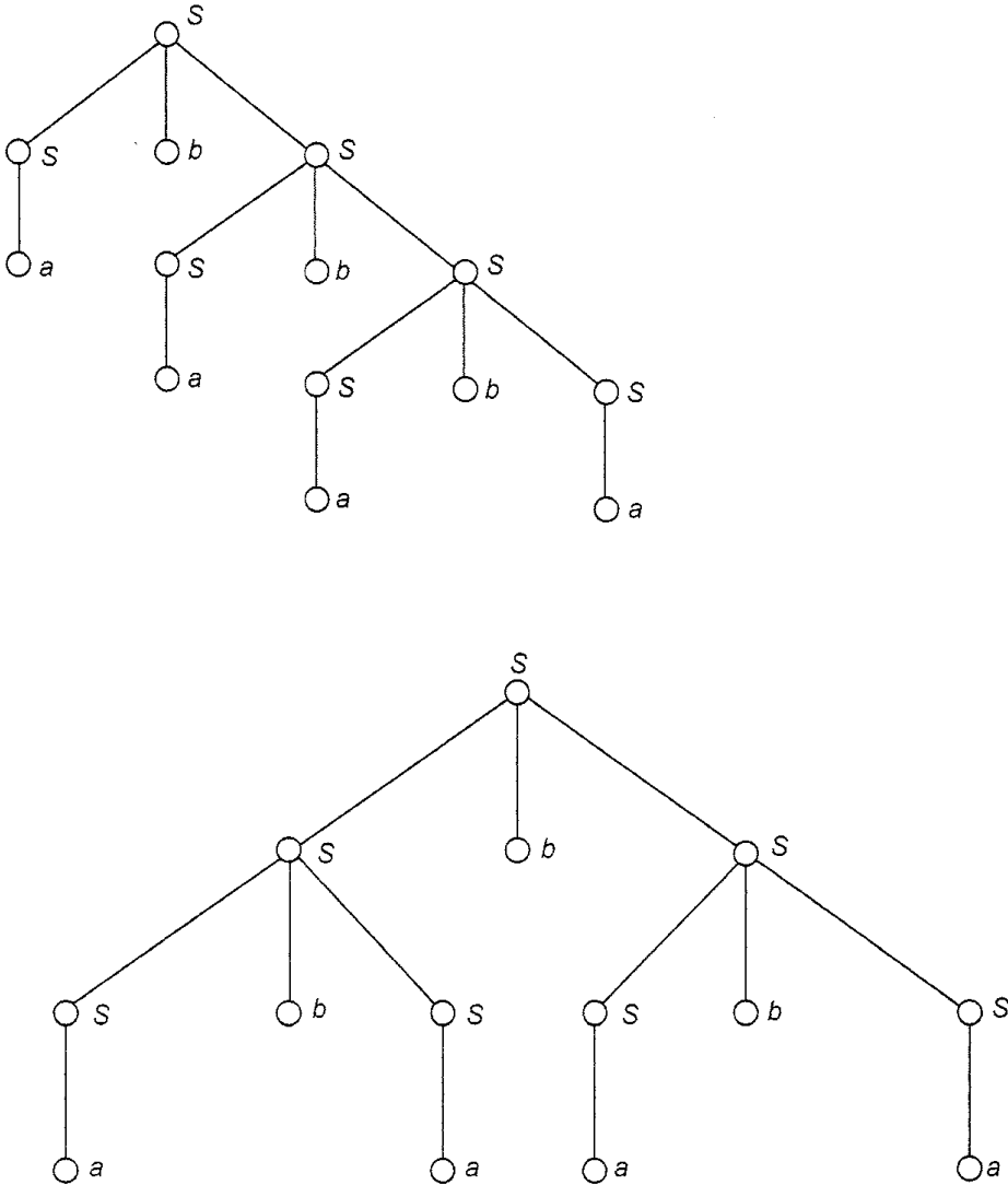
Fig. 6.11 Two derivation trees of abababa for Example 6.4.
