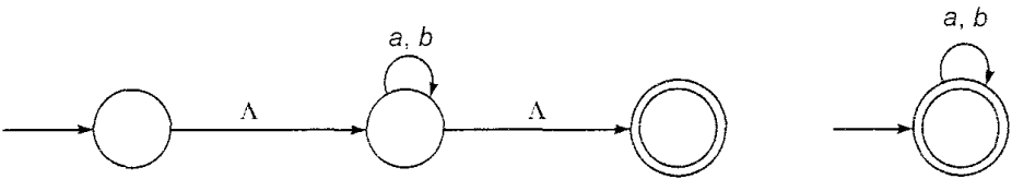
Fig. 5.25 Transition system for (a + b)^* .
