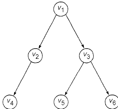
Fig. 2.8 An ordered directed tree.
