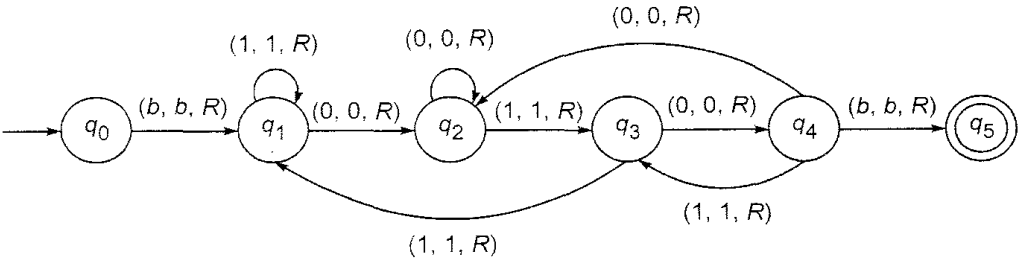
Fig. 9.13 TM for Example 9.14.
