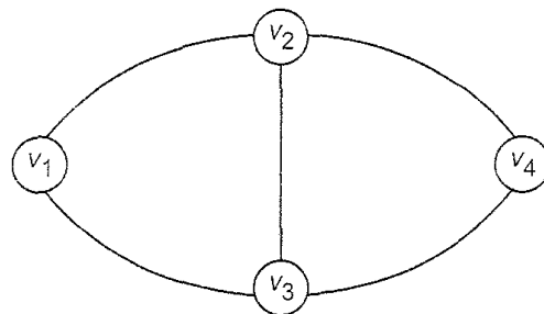
Fig. 2.5 A graph.
