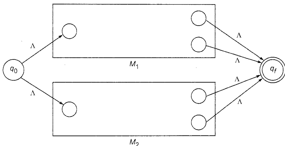
Fig. 5.7 NFA accepting L(P + Q) .
