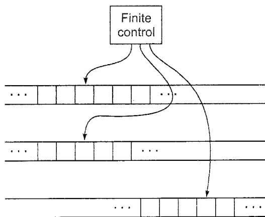
Fig. 9.8 Multitape Turing machine.
