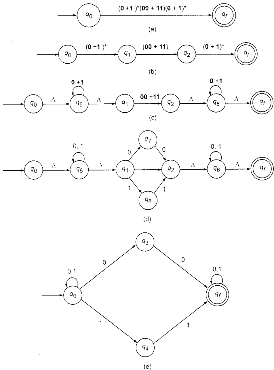
Fig. 5.18 Construction of finite automaton equivalent to (0 + 1)^*(00 + 11)(0 + 1)^* .
