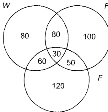
Fig. 2.17 Venn diagram for Example 2.27.
