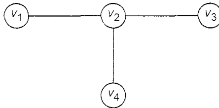
Fig. 2.6 A tree with four vertices.
