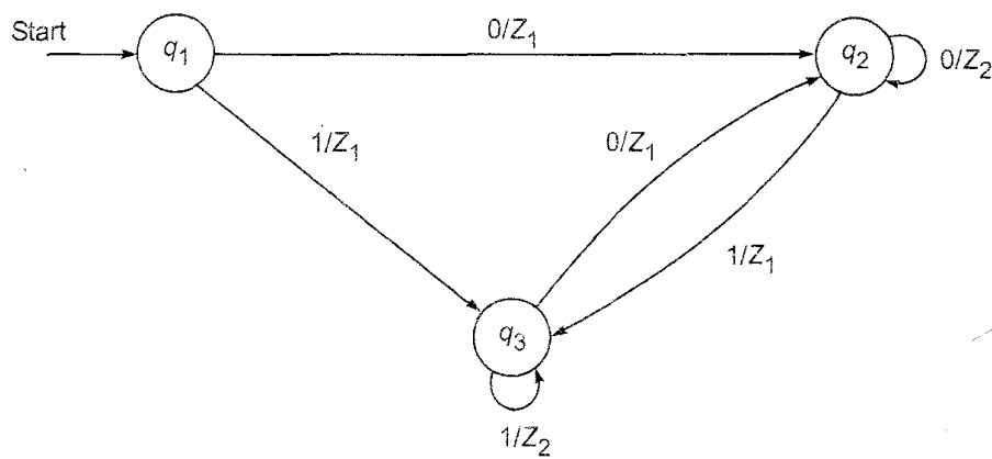
Fig. 3.10 Mealy machine of Example 3.12.
