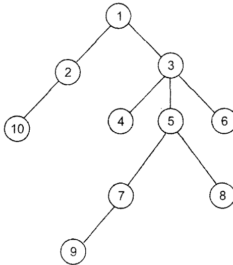
Fig. 2.13 The directed tree for Example 2.18.
