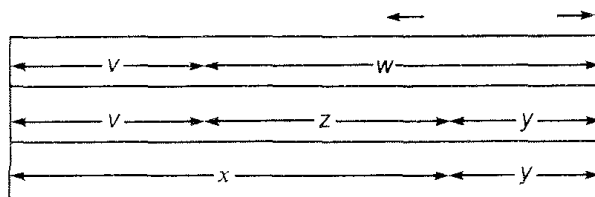
Fig. 2.14 Illustration of Levi's theorem.
