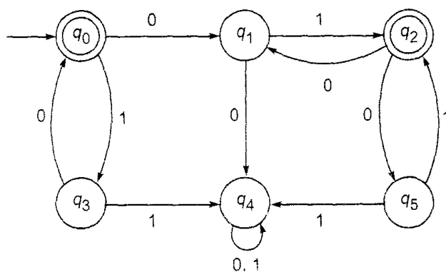
Fig. 3.22 DFA of Exercise 3.16.
