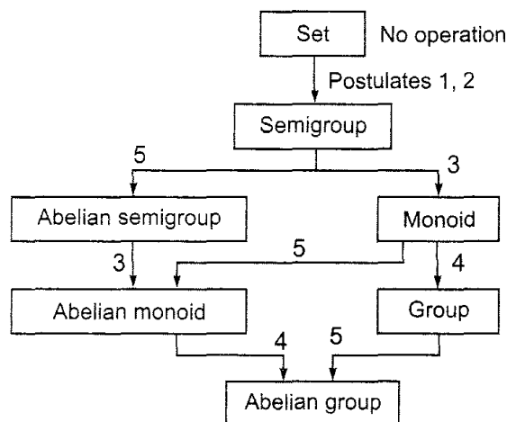
Fig. 2.1 Sets with one binary operation.
