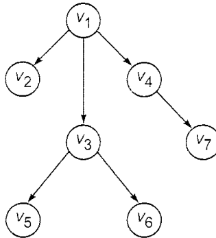
Fig. 2.7 A tree with seven vertices.
