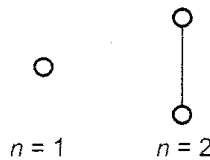
Fig. 2.15 Trees with one or two vertices.
