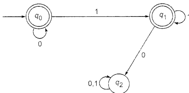
Fig. 5.29 Finite automaton of Example 5.23.
