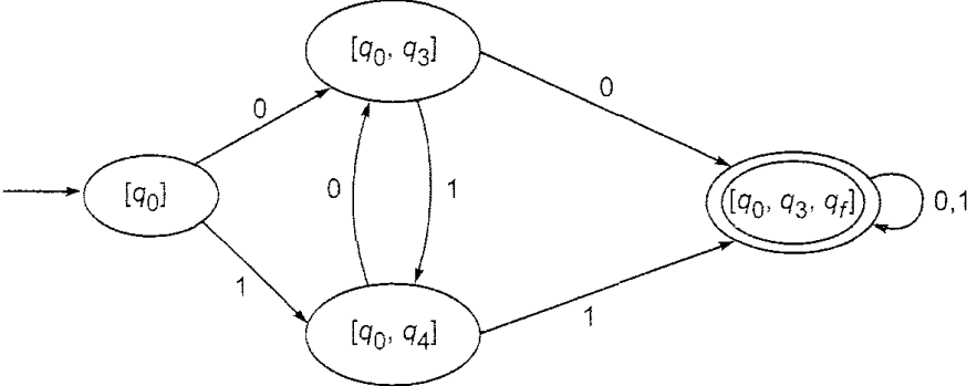
Fig. 5.20 Reduced finite automaton of Example 5.13.
