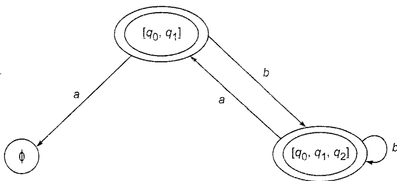
Fig. 5.12 Deterministic transition system for Example 5.7.
