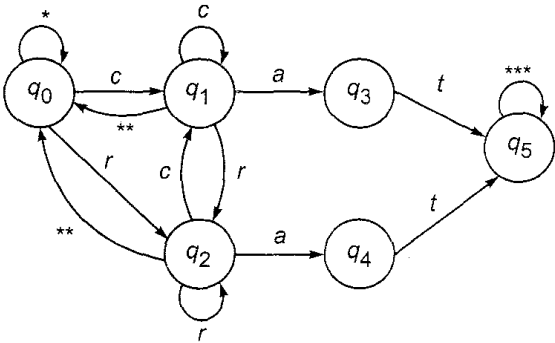
Fig. A3.2 Transition system for Exercise 3.10
