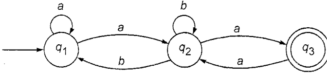
Fig. 5.13 Transition system of Example 5.8.
