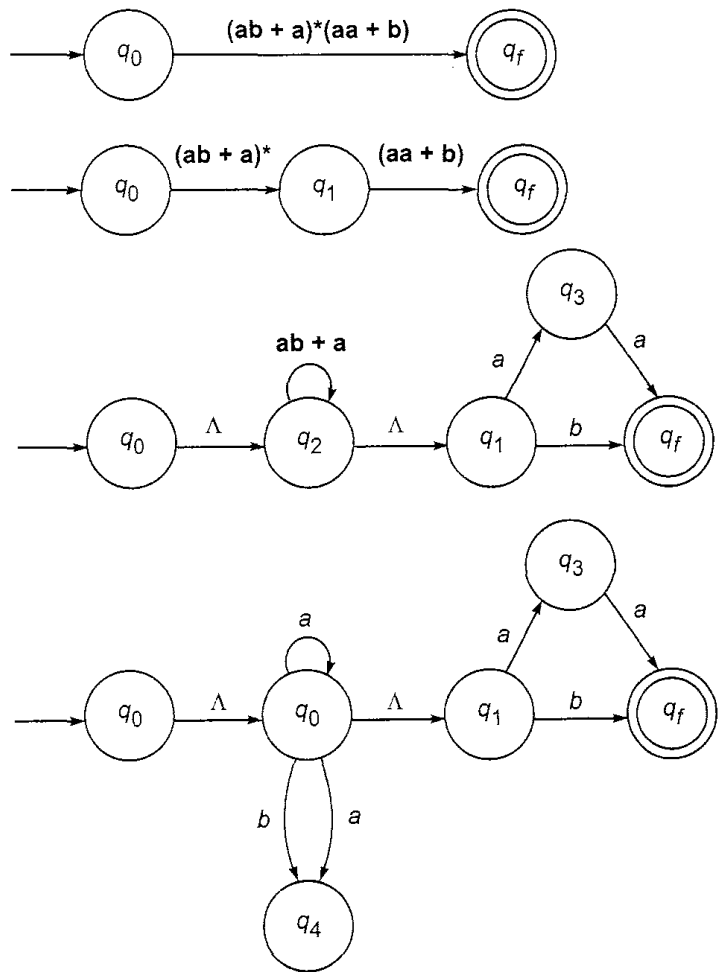
Fig. A5.1 Transition system for Exercise 5.5.
