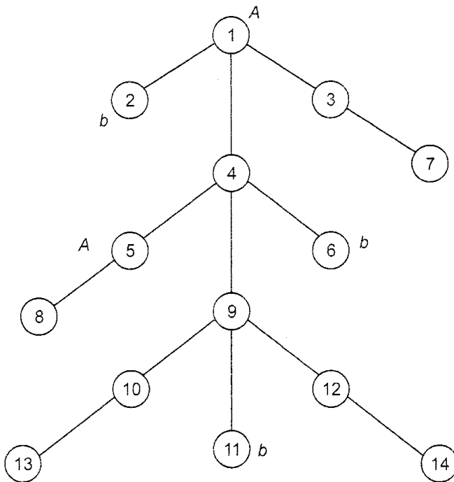
Fig. 6.14 Derivation tree for Question 1(e).
