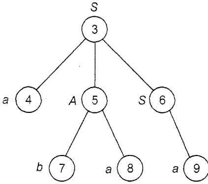
Fig. 6.2 A subtree of Fig. 6.1.
