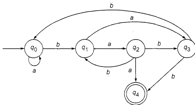
Fig. 5.36 NDFSA for Example 5.36.
