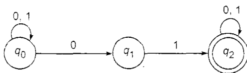
Fig. 3.21 Automaton for Statements 6–15.
