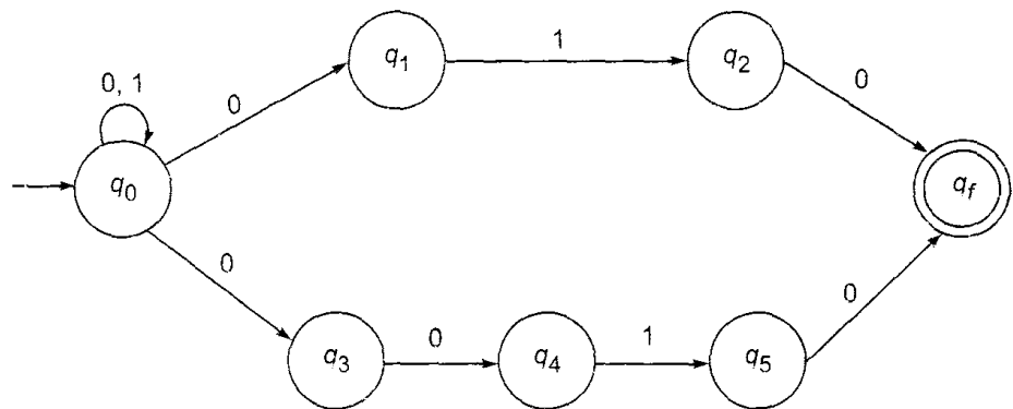
Fig. A5.4 N DFA for Exercise 5.12.
