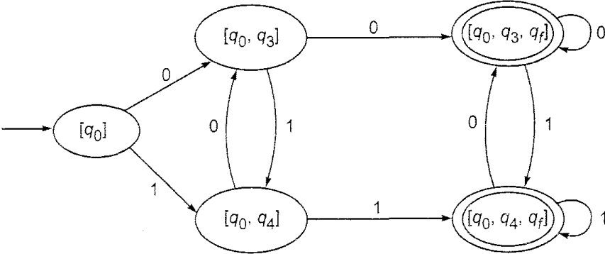
Fig. 5.19 Finite automaton of Example 5.13.
