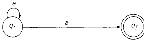
Fig. 5.34 Transition system for Example 5.26.
