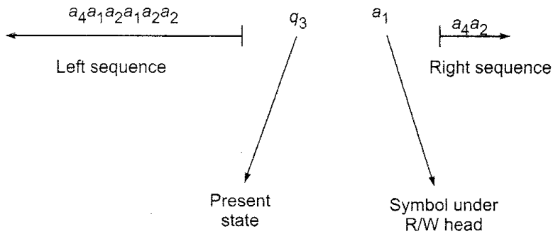
Fig. 9.3 Representation of ID.
