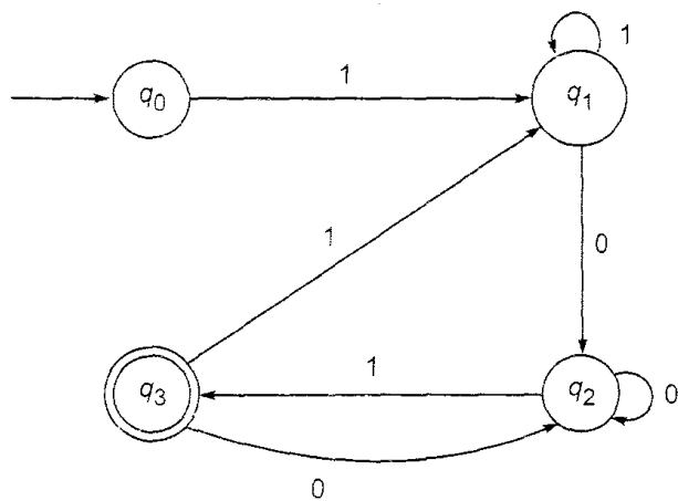
Fig. 5.38 Transition system of Exercise 5.8.
