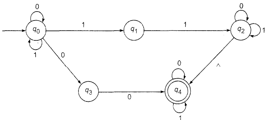
Fig. 3.8 Transition system for a nondeterministic automaton.
