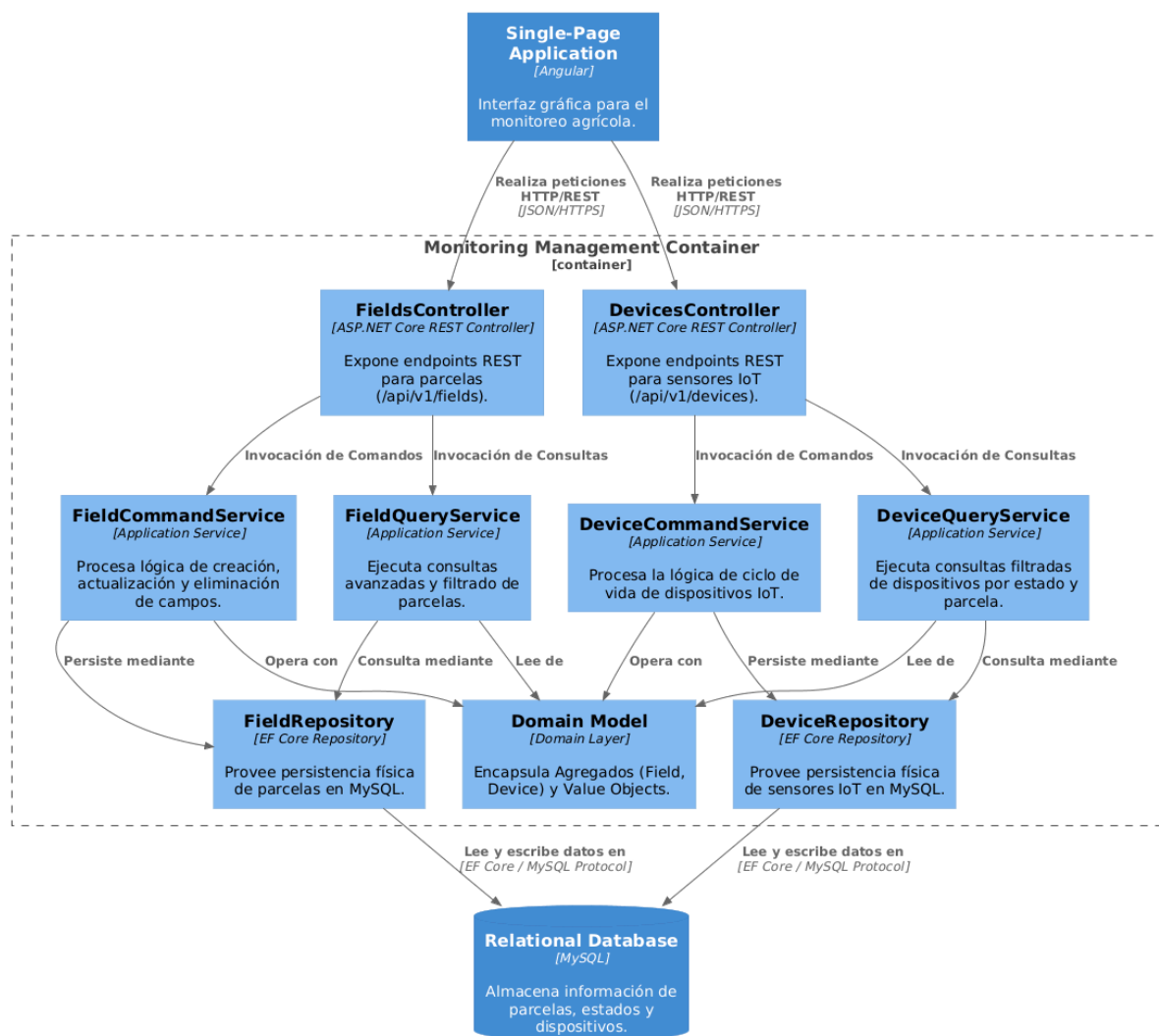
Component Diagram for Monitoring Management Bounded Context
