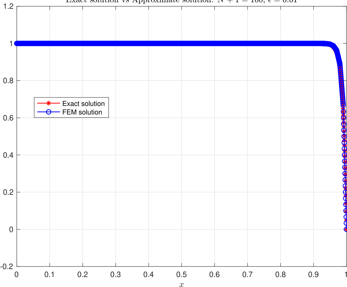
Exact solution vs Approximate solution: N + 1 = 100 , \epsilon = 0.01
