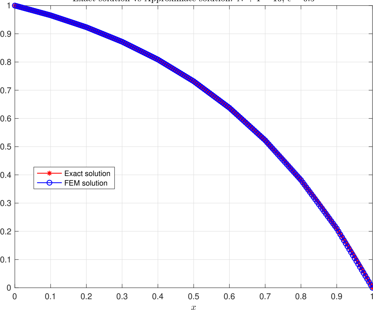
Exact solution vs Approximate solution: N + 1 = 10 , \epsilon = 0.5
