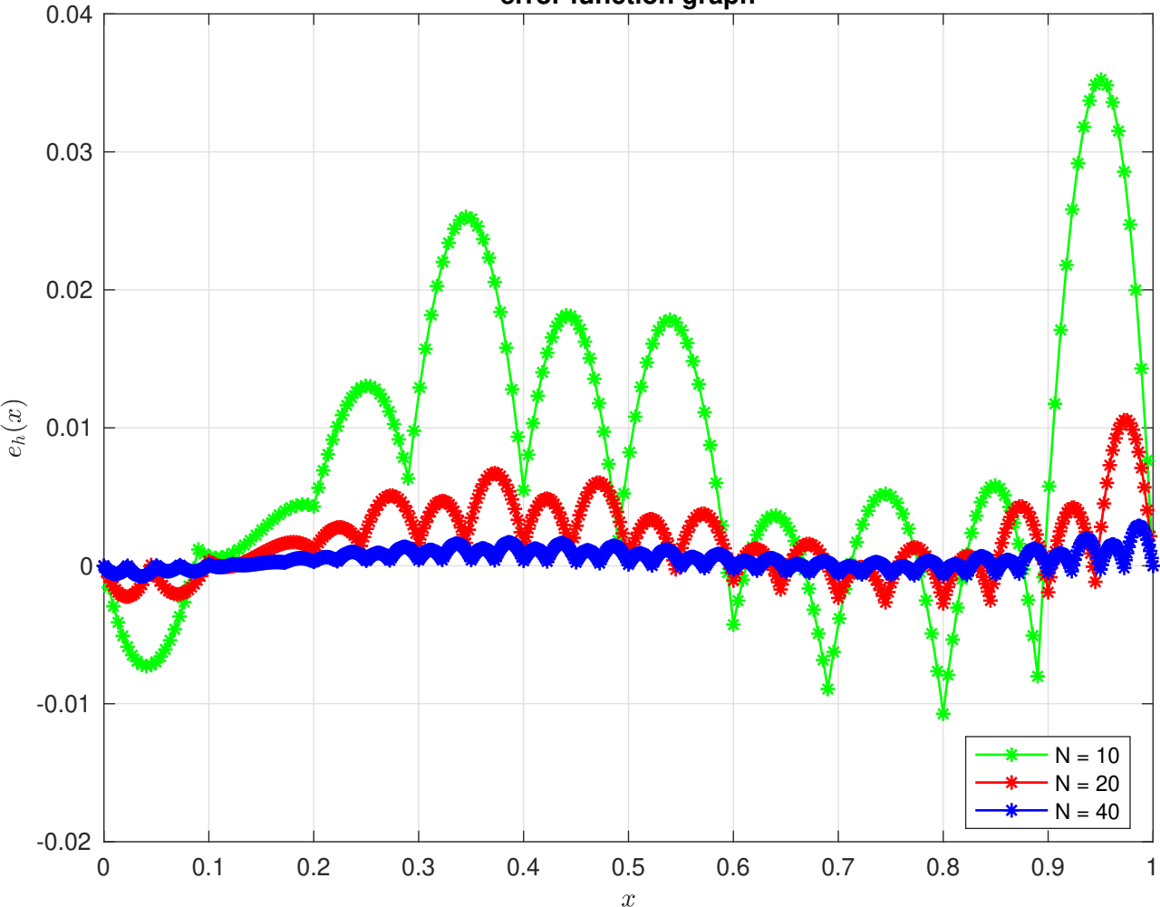
error function graph
