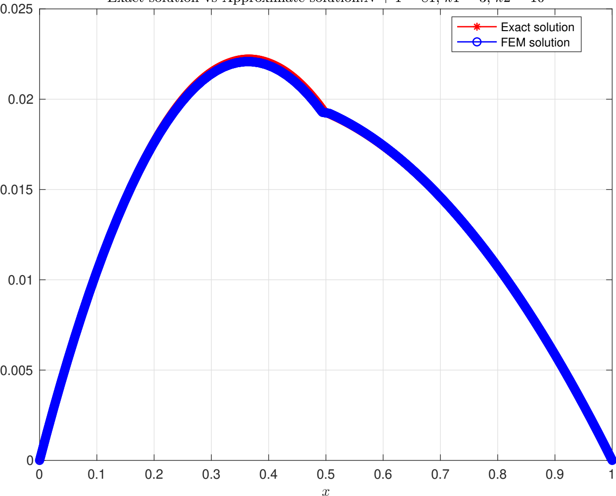
Exact solution vs Approximate solution: N + 1 = 81 , k_1 = 3 , k_2 = 10
