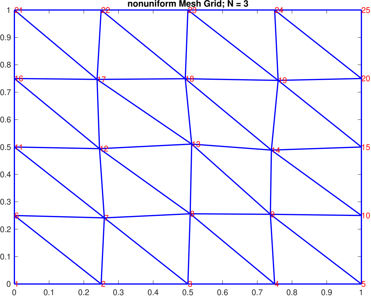
nonuniform Mesh Grid; N = 3
