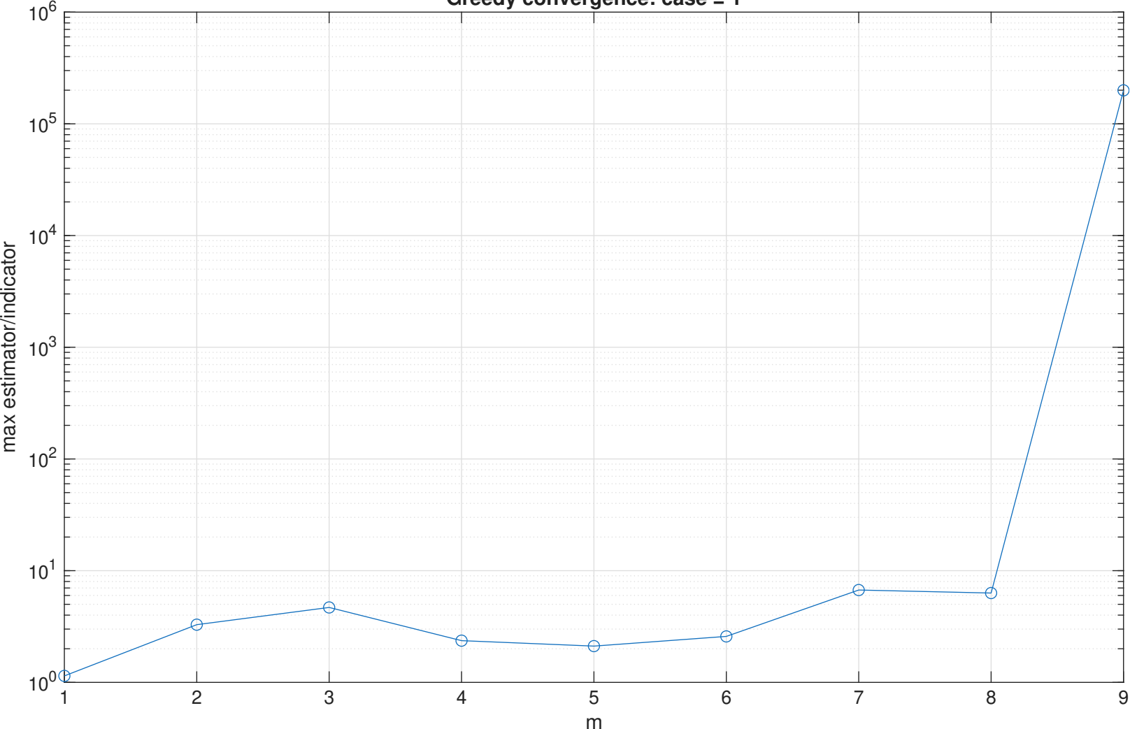
Greedy convergence: case = 1
