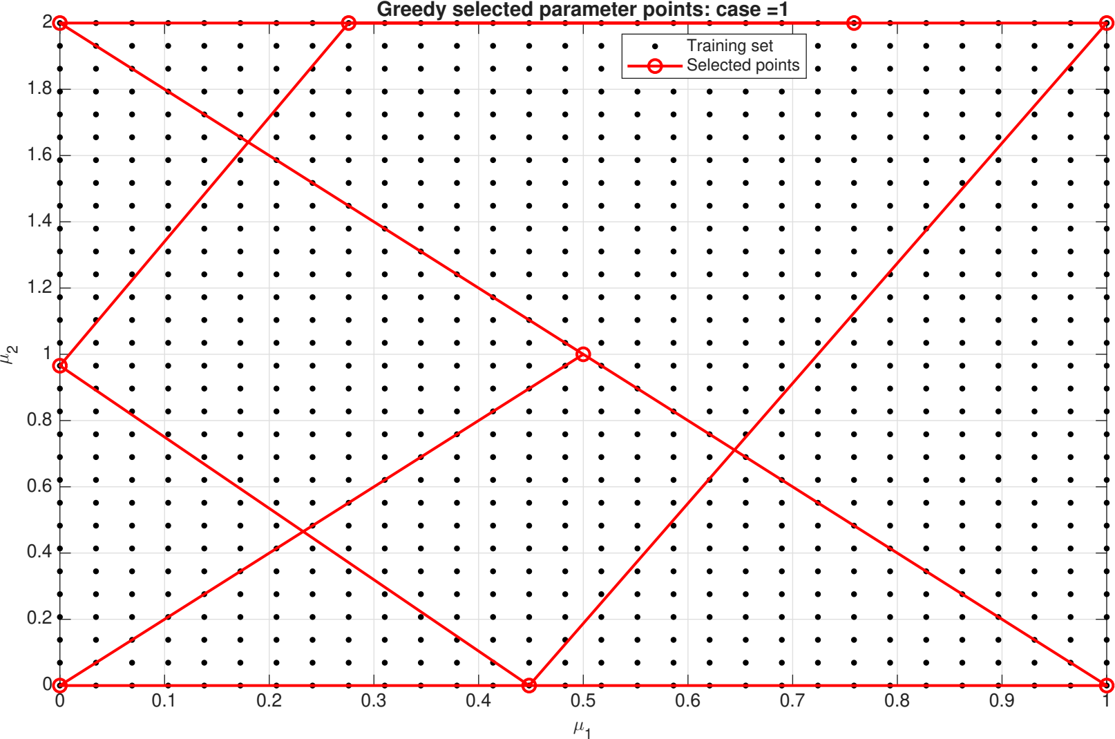
Greedy selected parameter points: case =1
