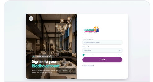
User Login
