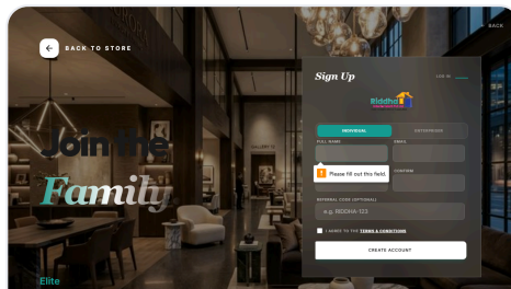
Signup Validation
