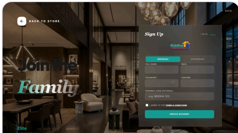
Signup
