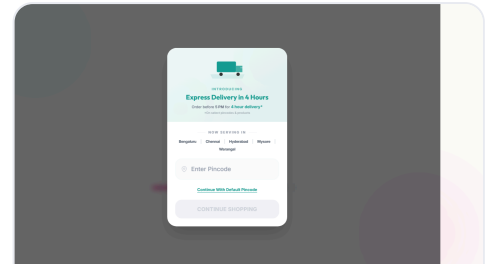
Homepage – Modal Blocking
