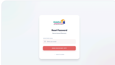
Forgot Password
