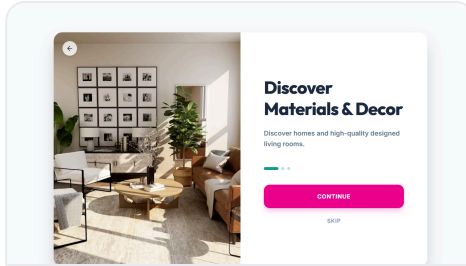
Onboarding
