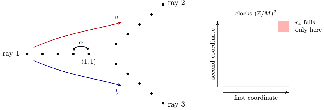
Figure 1: Left: Houghton's group H_3 acts on three rays of points. The generator a translates along rays 1 and 2: points of ray 1 move toward the centre and on into ray 2. The generator b does the same with rays 1 and 3, and \alpha swaps the first two points of ray 1. Right: a corner model (Section 4.2) follows the quotient \mathbb{Z}^2 on a clock torus (\mathbb{Z}/M)^2 and colours the points. The relation r_4 = aba^{-1}b^{-1}\alpha^{-1} fails only over one corner clock, a fraction M^{-2} of the model, whose size is \exp(O(M)) .
