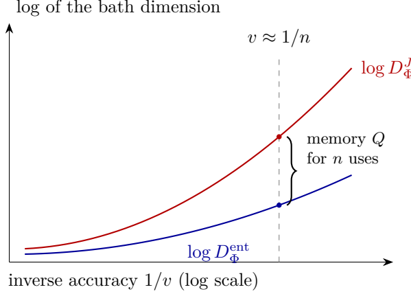
Figure 2: Theorem B in a picture. The memory for n uses lies between two profiles read at accuracy about 1/n : below, the one-round profile, which allows biased bath states and measures leakage; above, the Choi profile of single exact factors. For \Phi_H the one-round profile at distance 1/8 is between \exp(c v^{-\beta_H}) and \exp(O(v^{-1/3})) (Proposition 4.17), and the Choi profile is at most \exp(O(v^{-1/3} \log^{4/3}(1/v))) (Theorem 3.36).
