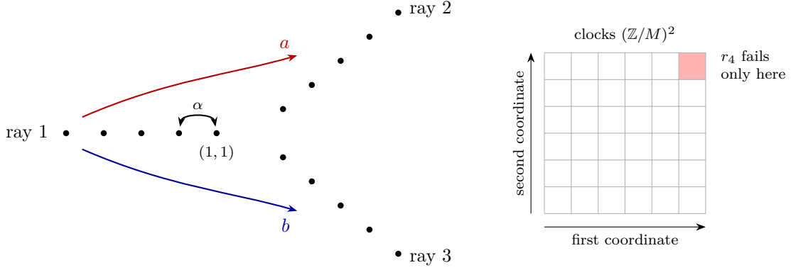
Figure 3: Left: Houghton's group H_3 acts on three rays of points. The generator a translates along rays 1 and 2: points of ray 1 move toward the centre and on into ray 2. The generator b does the same with rays 1 and 3, and \alpha swaps the first two points of ray 1. Right: a corner model (Section 4.3) follows the quotient \mathbb{Z}^2 on a clock torus (\mathbb{Z}/M)^2 and colours the points. The relation r_4 = aba^{-1}b^{-1}\alpha^{-1} fails only over one corner clock, a fraction M^{-2} of the model, whose size is \exp(O(M)) .
