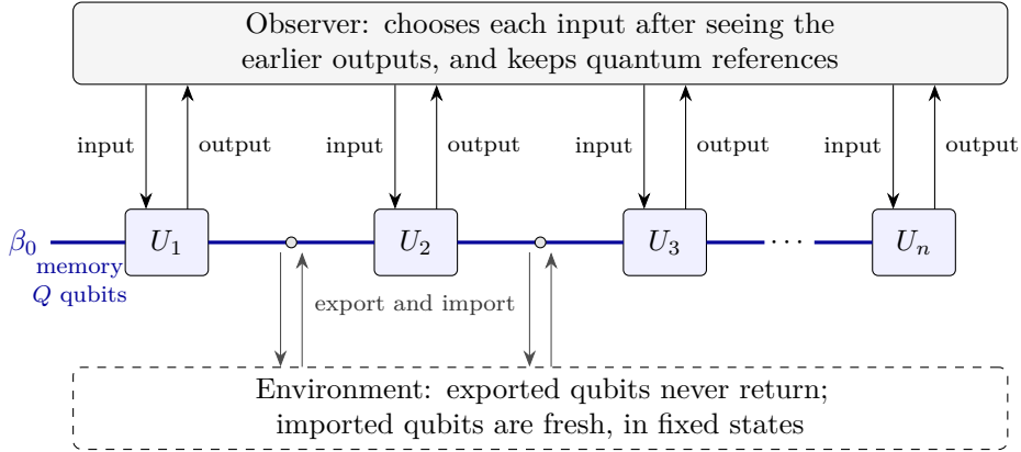
Figure 1: Causal service of a channel for n rounds. The memory (thick line) starts in a fixed state \beta_0 . In each round a fixed unitary U_t acts on the fresh input and the memory, and the output is released at once. Between rounds some memory qubits are exported for good and replaced by fresh imports. The observer may adapt each input to everything seen so far.
