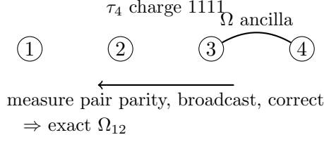
Figure 2: Puncturing: pairing charged holders 3, 4 with a declared \Omega ancilla and measuring the pair parities lowers the charge 1111 to 1100, leaving an exact reference on holders 1, 2 after the heralded sign correction.
