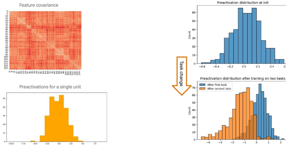
Figure 7.3: How a large step kills a unit, from the Continual Learning lecture. Left, the feature covariance the network has built up and the preactivation histogram for one unit. Right, the same unit’s preactivation distribution at initialisation, centred on zero and narrow, and after training on two tasks: the second task’s distribution, in orange, has shifted almost entirely below zero. Once preactivations leave the range where the activation responds, the unit stops passing gradient, which is what “the ReLUs are dead” means in practice.
