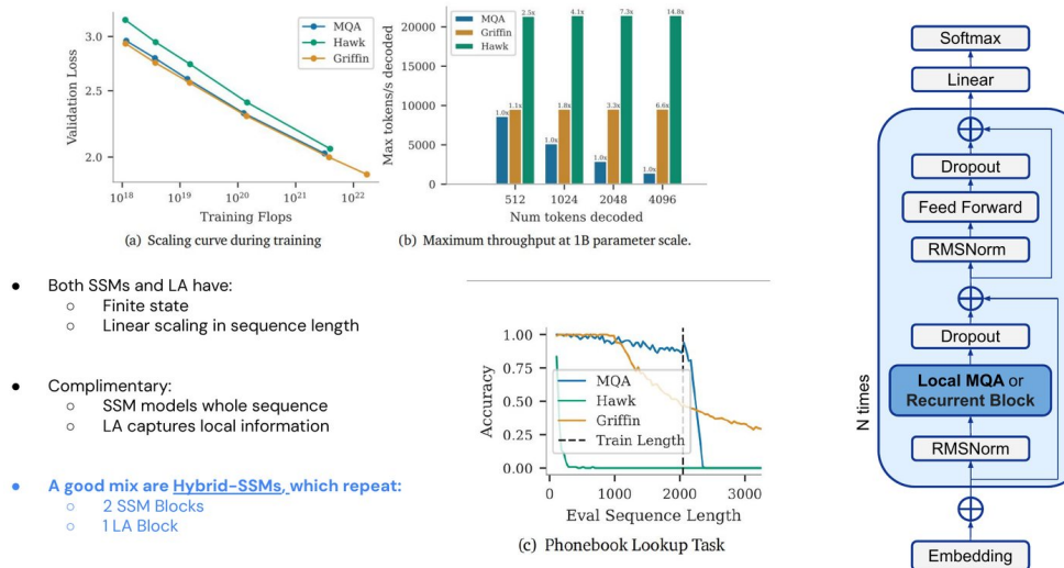
Figure 8.3: What actually wins, from the To Be Figured Out lecture. Left, the case for hybrids: state space models and linear attention share a finite state and linear scaling in sequence length, and are complementary because the SSM models the whole sequence while linear attention captures local structure. Middle, the evidence, with matched scaling curves, an order-of-magnitude throughput advantage at 1B parameters, and a phonebook-lookup task where the pure recurrent variants degrade past their training length. Right, the resulting block, alternating a recurrent or local-attention block with feed-forward layers.
