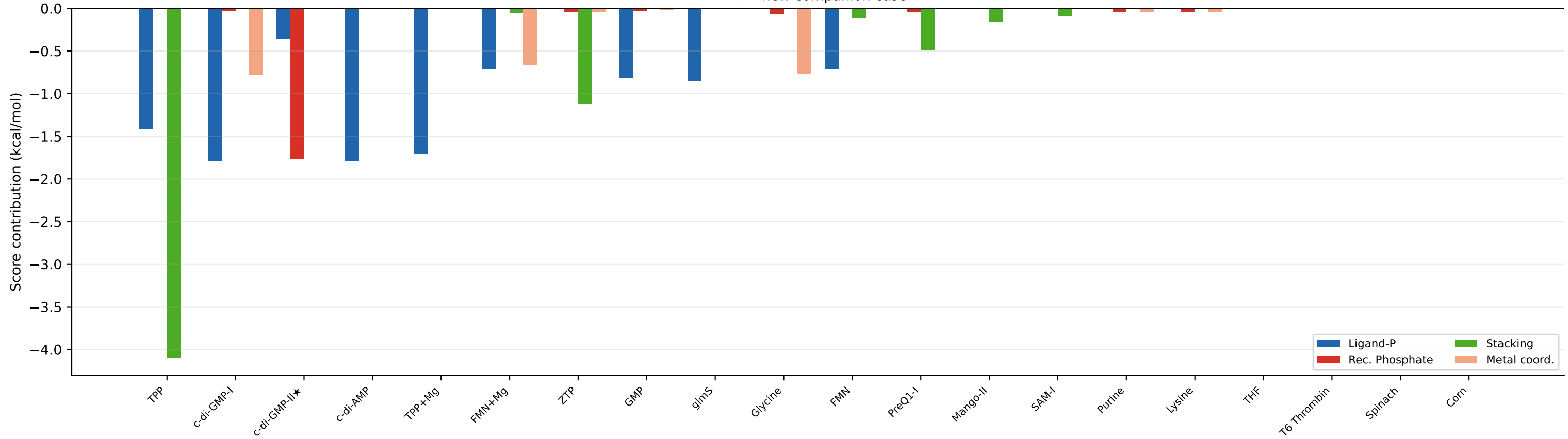
Aptamer scoring term breakdown per case (crystal pose)
