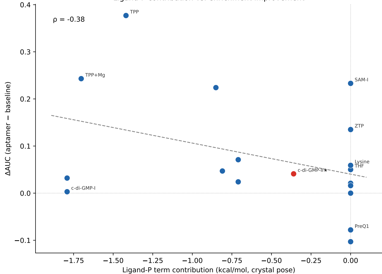
Ligand-P contribution vs. enrichment improvement
