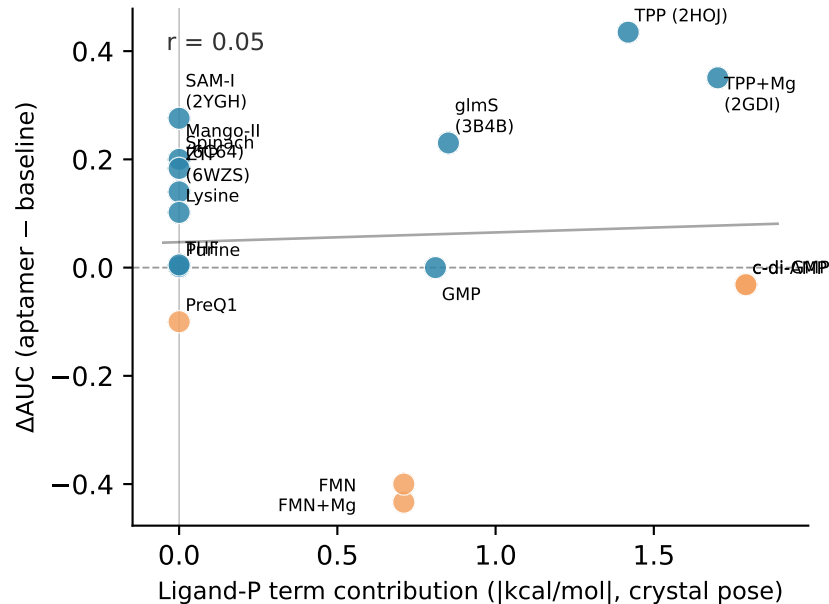
Phosphate contribution vs. enrichment improvement
