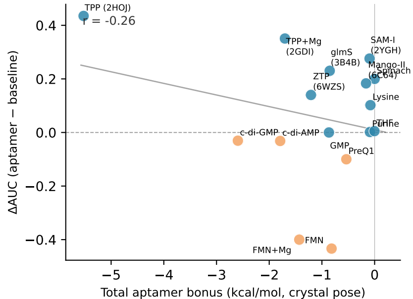
Total aptamer score vs. enrichment improvement
