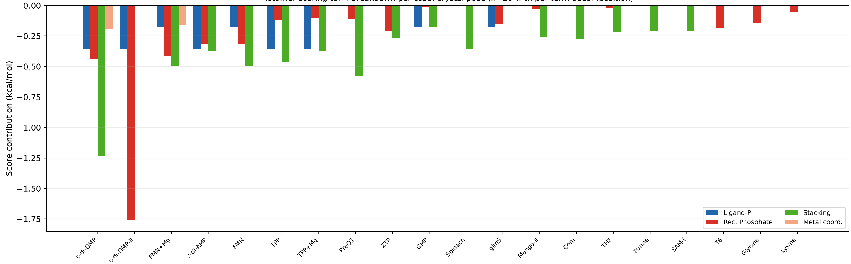
Aptamer scoring term breakdown per case, crystal pose (n=20 with per-term decomposition)
