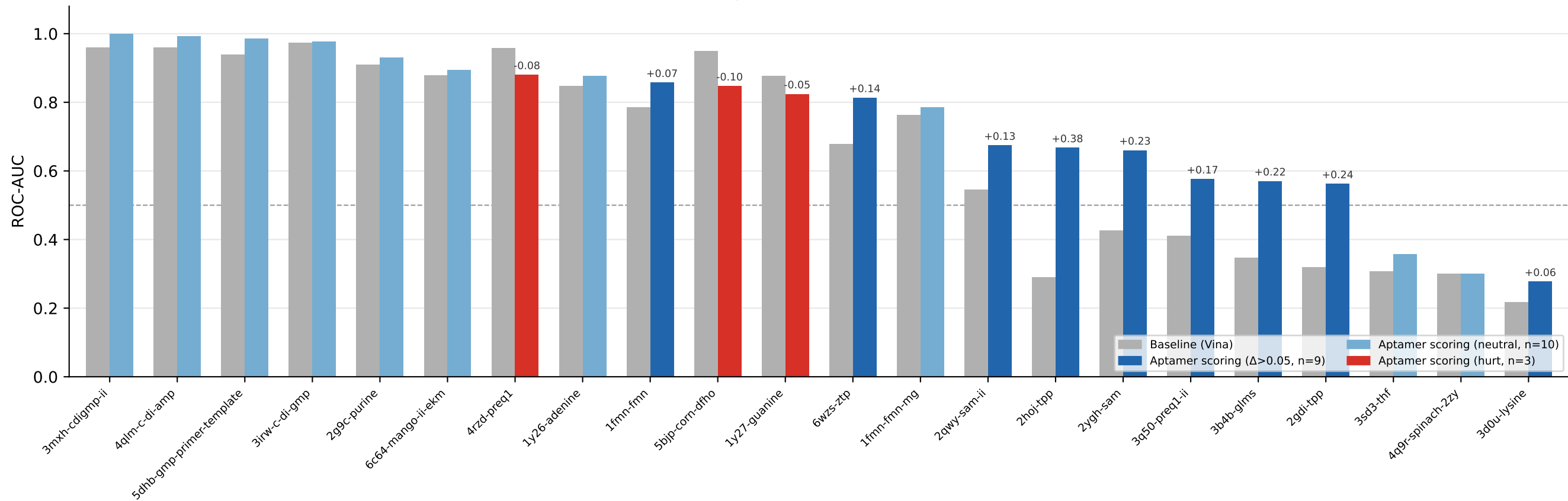
RNA aptamer VS benchmark — 22 enrichment cases Aptamer scoring vs. baseline Vina | 9/22 help 10/22 neutral 3/22 hurt mean \Delta\text{AUC}=+0.076
