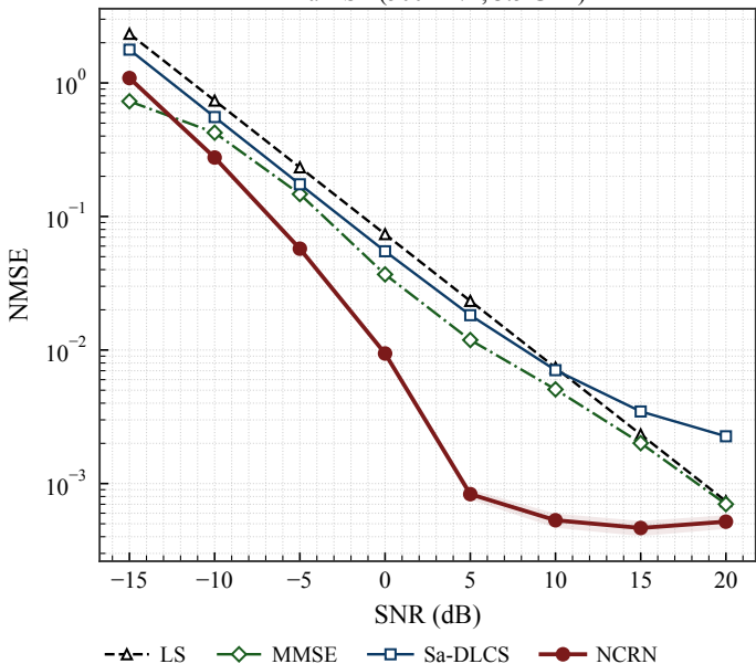
RMa HST (500 km/h, 3.5 GHz)
