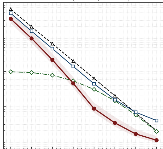
RMa NLOS (300 km/h, 3.5 GHz)
