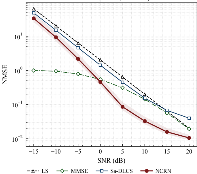
UMi O2I (3 km/h, 28.0 GHz)
