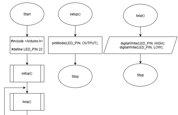
Gambar 4-2-1 Flowchart Source Code Percobaan 2
