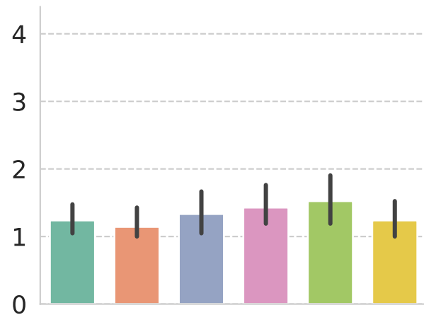
Falcon 3 (1B)
