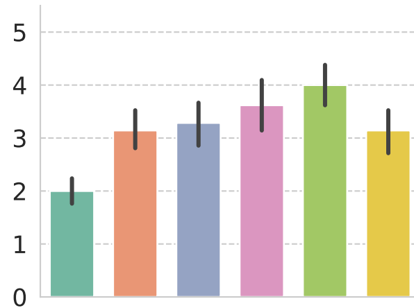
Qwen 3 (0.6B)
