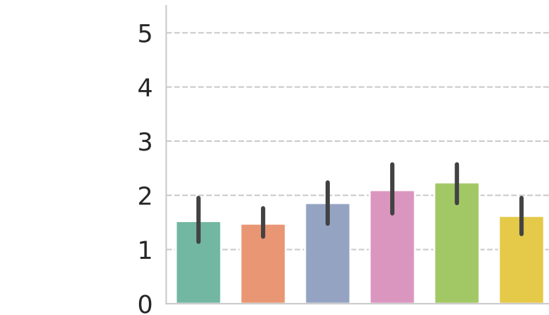
SmolLM2 (1.7B)
