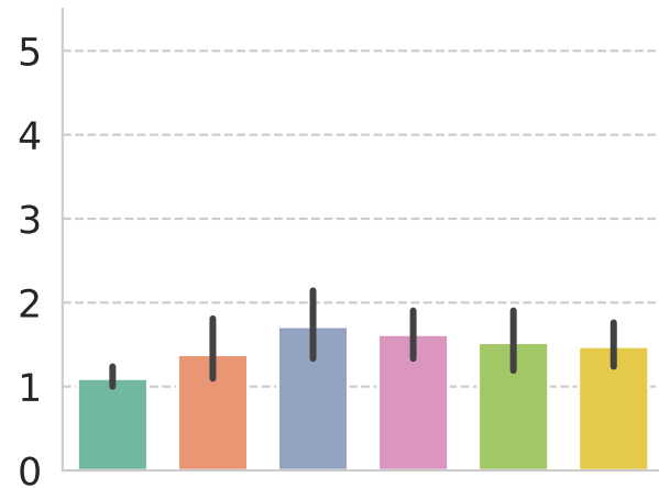
Qwen 2.5 (0.5B)
