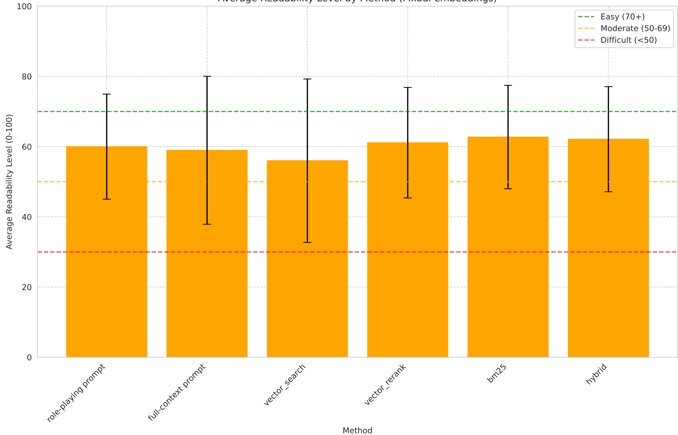
Average Readability Level by Method (Mxbai embeddings)
