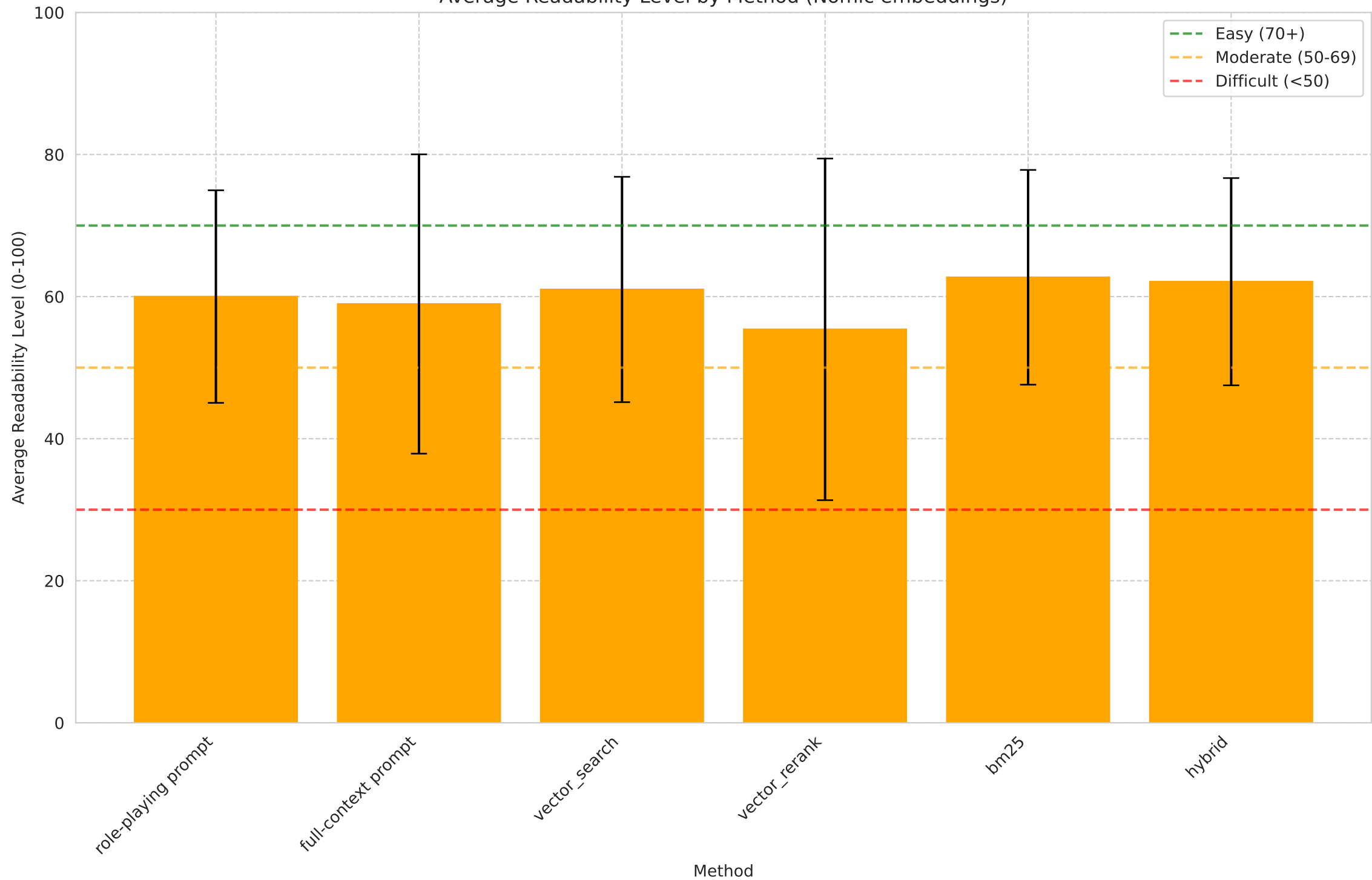
Average Readability Level by Method (Nomic embeddings)
