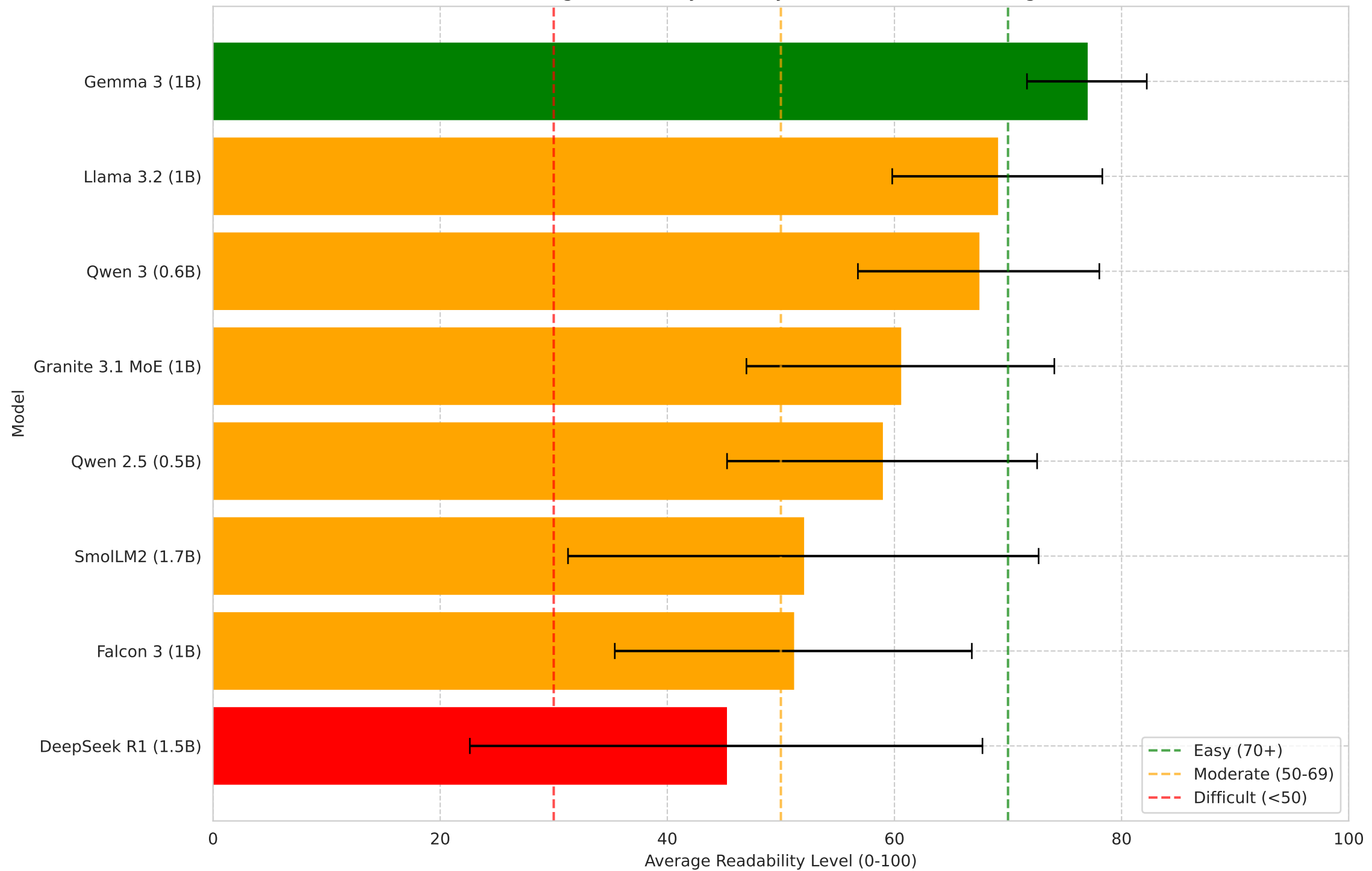
Average Readability Level by Model (Mxbai embeddings)
