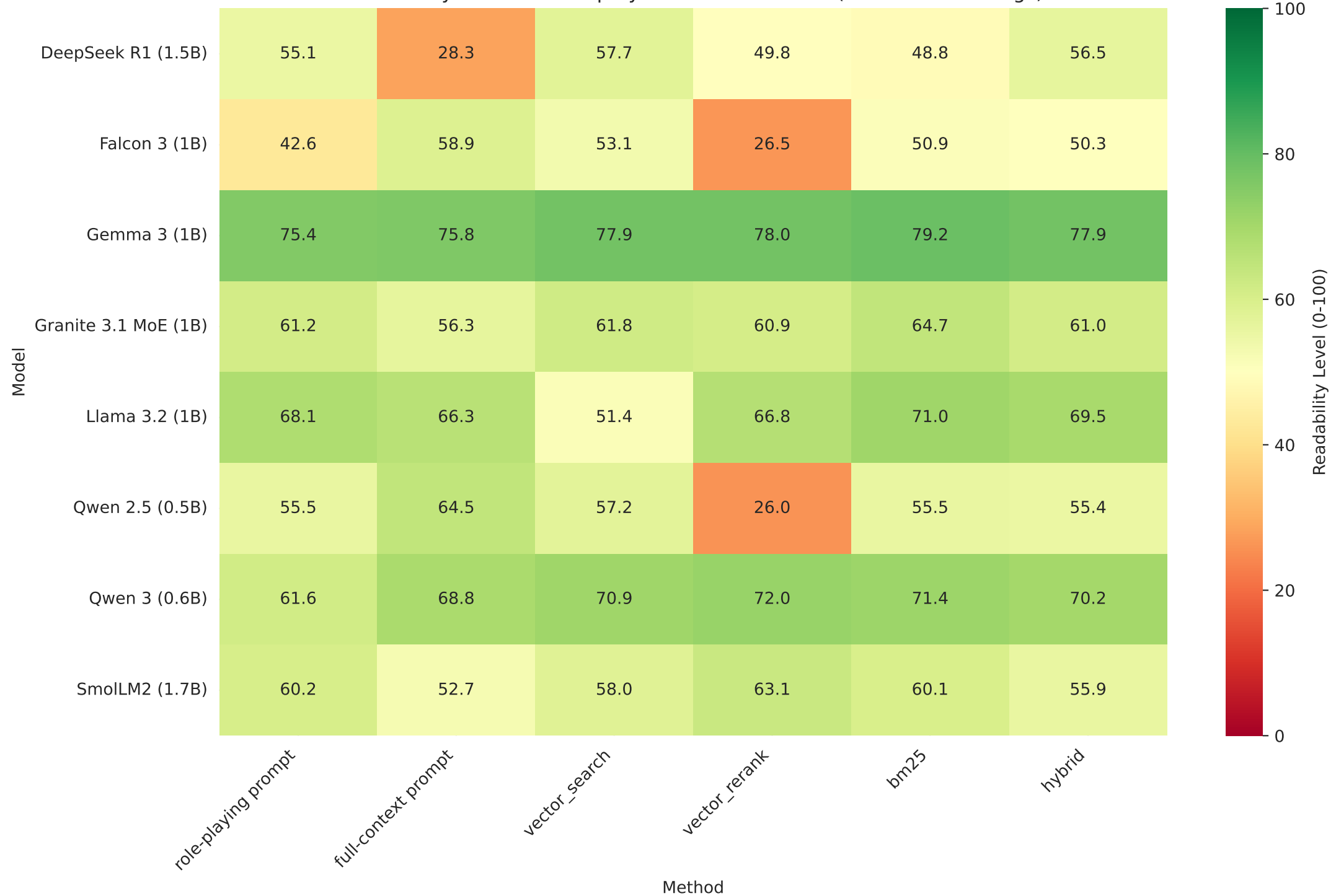
Readability Level Heatmap by Model and Method (Nomic embeddings)
