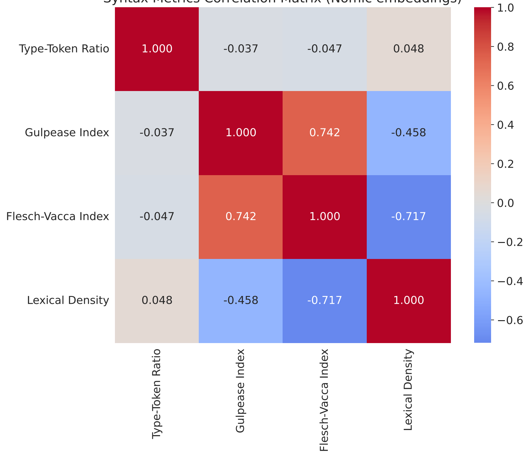
Syntax Metrics Correlation Matrix (Nomic embeddings)
