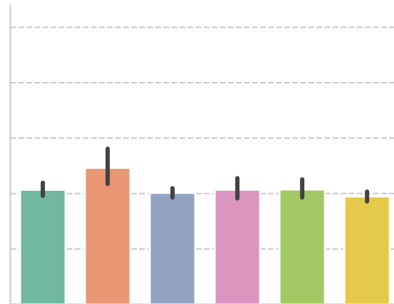
Falcon 3 (1B)
