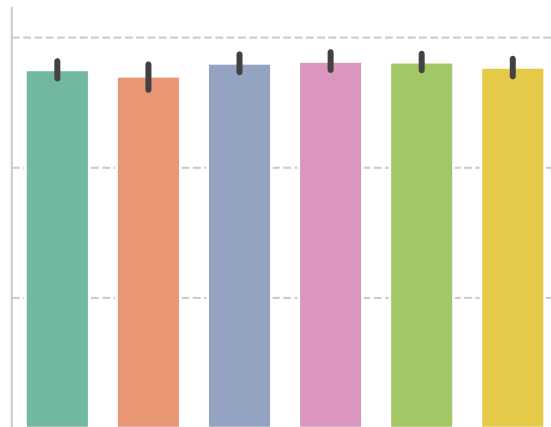
Qwen 2.5 (0.5B)
