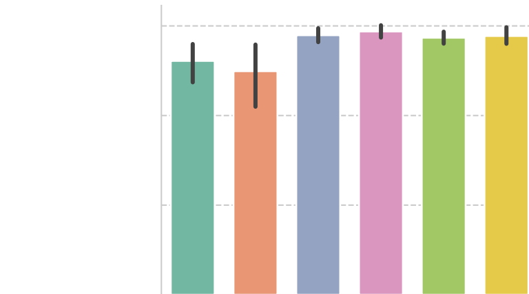
SmolLM2 (1.7B)
