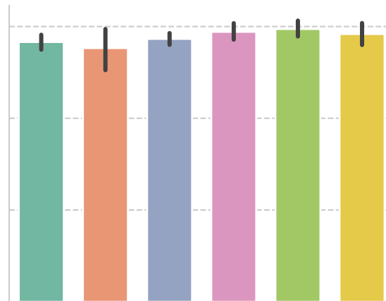
Qwen 3 (0.6B)
