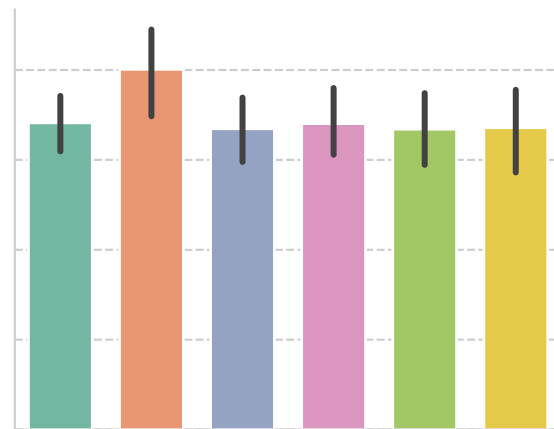
Falcon 3 (1B)
