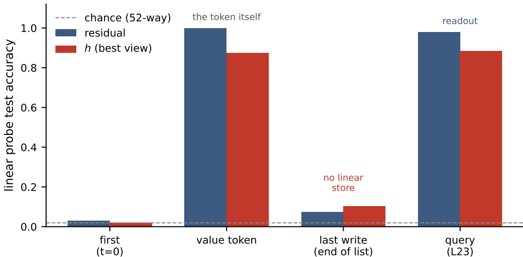
Store \neq readout: last-write has no linear value code (n=384, not v1)
