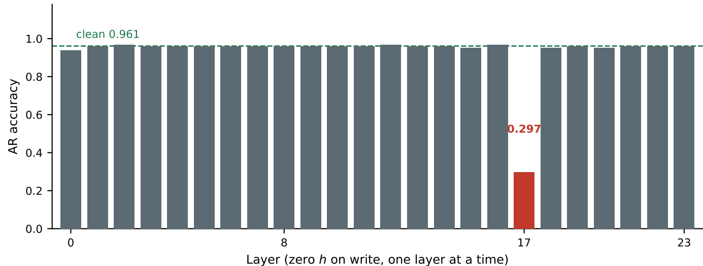
Only layer 17 write-wipe collapses associative recall (n=128)
