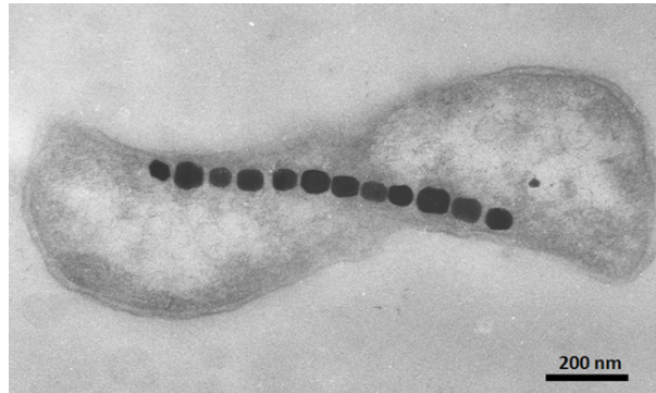
Figuur 2: Magnetosoom ketting in bacterium[14]
