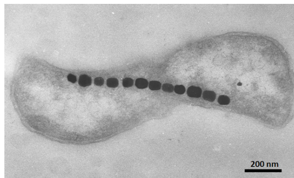
Figuur 5 – Magnetosoom ketting in bacterium [16]
